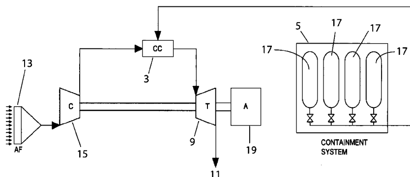
Fig 2: Plant's Scheme (AF = Air Filter, C = Compressor, CC = Combustion Chamber, T = Turbine, A = Alternator)
