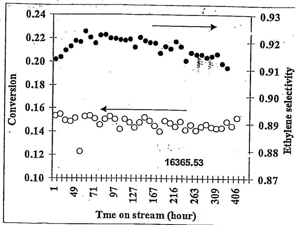
Figure 2B: Ethane conversion and ethylene selectivity over 400 hours for \text{Ni}_{0.71}\text{Nb}_{0.27}\text{Co}_{0.02}\text{O}_x over at 275 °C.
