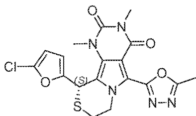
(S)-10-(5-chlorofuran-2-yl)-1,3-dimethyl-5-(5-methyl-1,3,4-oxadiazol-2-yl)-7,8-dihydro-1H-pyrimido[4',5':3,4]pyrrolo[2,1-c][1,4]thiazine-2,4(3H,10H)-dione
