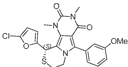
(S)-10-(5-chlorofuran-2-yl)-5-(3-methoxyphenyl)-1,3-dimethyl-7,8-dihydro-1H-pyrimido[4',5':3,4]pyrrolo[2,1-c][1,4]thiazine-2,4(3H,10H)-dione
