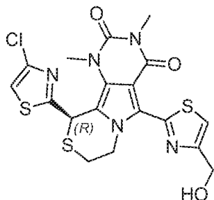
(R) -10-(4-chlorothiazol-2-yl)-5-(4-(hydroxymethyl)thiazol-2-yl)-1,3-dimethyl-7,8-dihydro-1H-pyrimido[4',5':3,4]pyrrolo[2,1-c][1,4]thiazine-2,4(3H,10H)-dione
