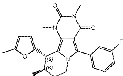
(9R,10S)-5-(3-fluorophenyl)-1,3,9-trimethyl-10-(5-methylfuran-2-yl)-7,8,9,10-tetrahydropyrimido[4,5-a]indolizine-2,4(1H,3H)-dione
