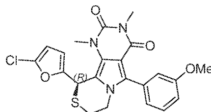
(R)-10-(5-chlorofuran-2-yl)-5-(3-methoxyphenyl)-1,3-dimethyl-7,8-dihydro-1H-pyrimido[4',5':3,4]pyrrolo[2,1-c][1,4]thiazine-2,4(3H,10H)-dione
