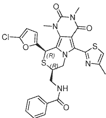
N-(((8R,10R)-10-(5-chlorofuran-2-yl)-1,3-dimethyl-5-(4-methylthiazol-2-yl)-2,4-dioxo-2,3,4,7,8,10-hexahydro-1H-pyrimido[4',5':3,4]pyrrolo[2,1-c][1,4]thiazin-8-yl)methyl)benzamide
