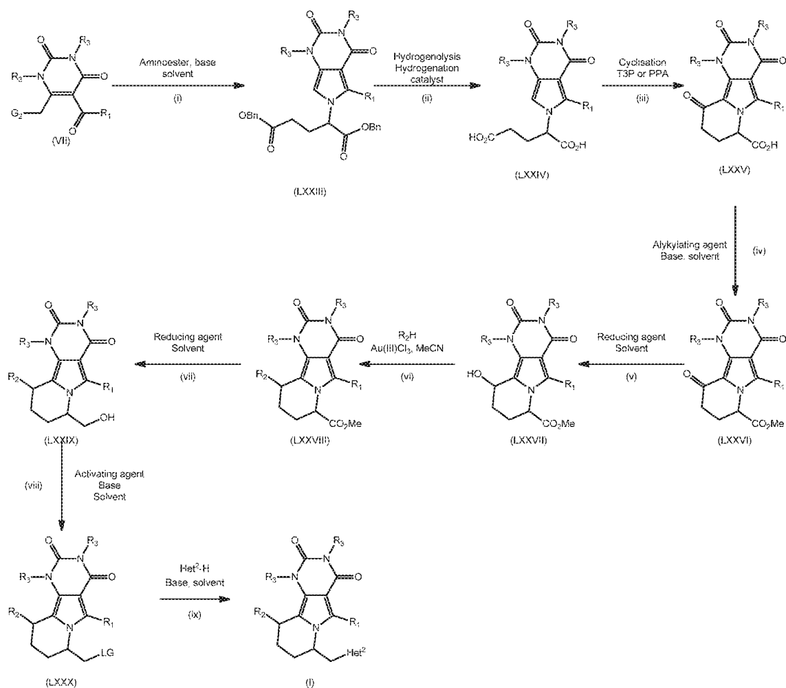
Scheme 21
