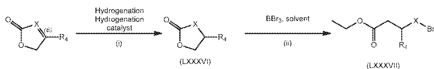
Scheme 23
