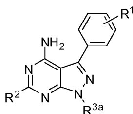
Formula (V);
