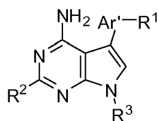
Formula (XI);
