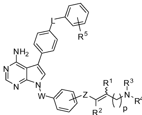
Formula (VIII);
