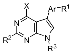
Formula (XIII);
