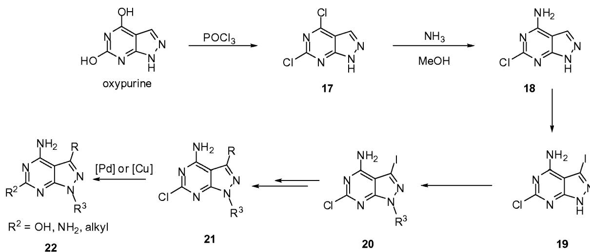
Scheme 4.
