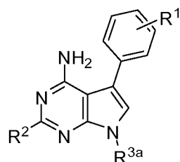
Formula (XIV);
