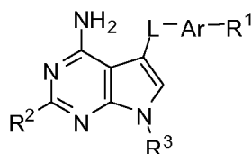
Formula (IX);
