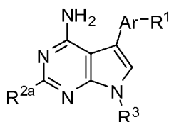
Formula (XII);
