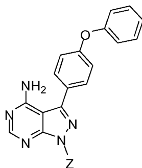
Formula (VIB);
