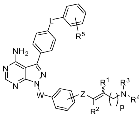
Formula (VII);
