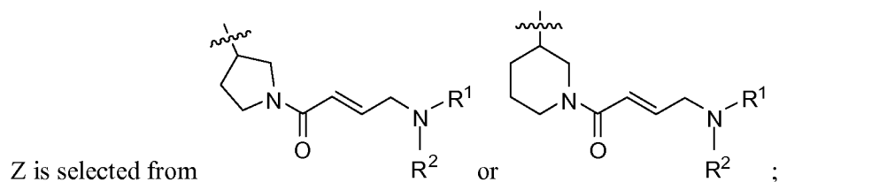
Formula (VIB);
