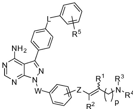
Formula (VII);
