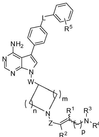
Formula (X);
