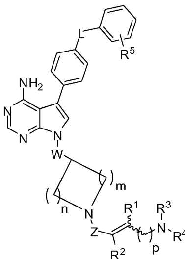
Formula (X);
