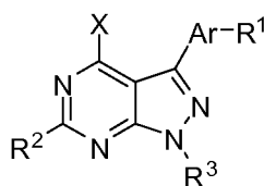
Formula (IV);
