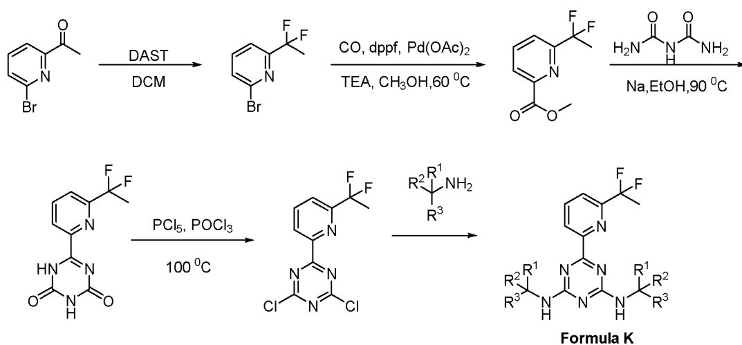
Scheme 9
