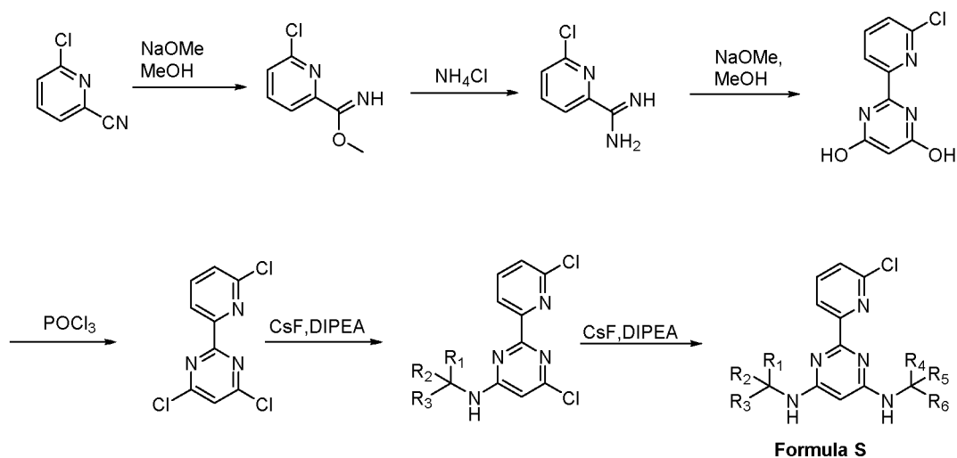
Scheme 32
