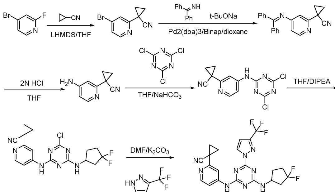
Scheme 36
