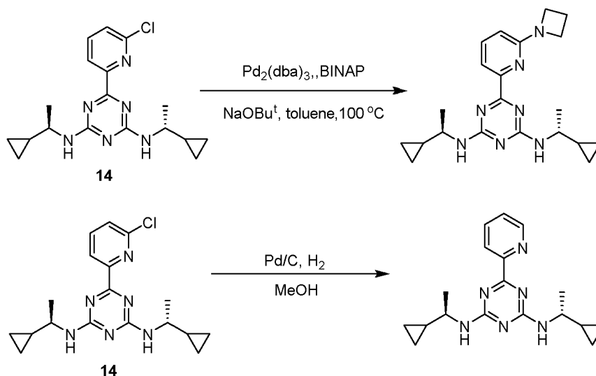
Scheme 5
