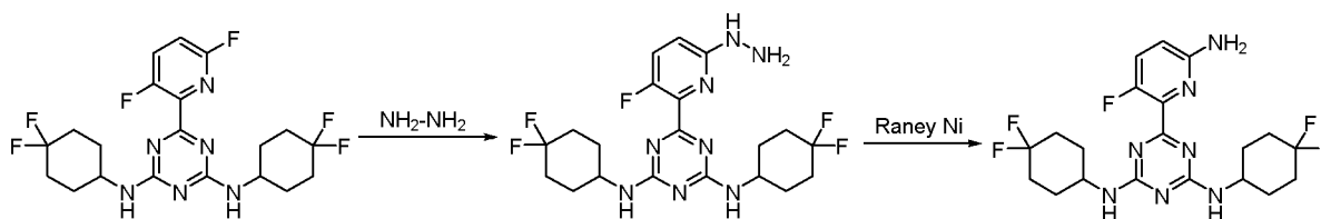
Scheme 17
