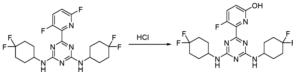
Scheme 18
