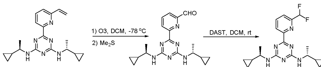
Scheme 14
