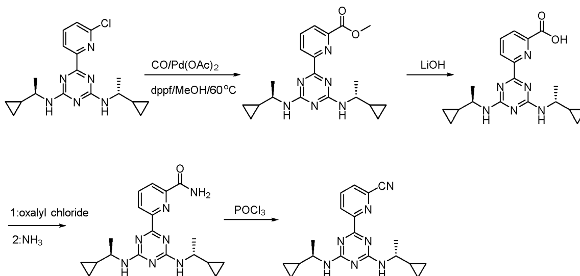
Scheme 15
