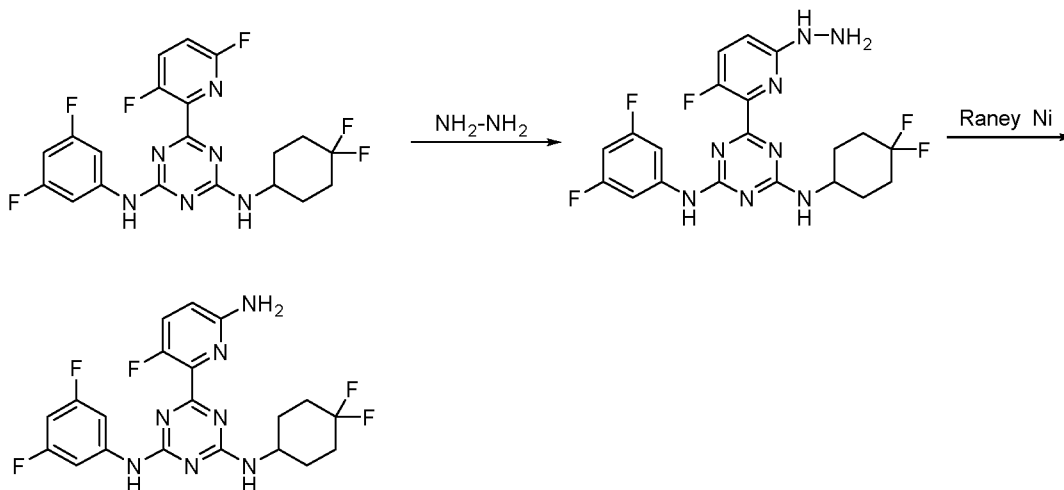
Scheme 34
