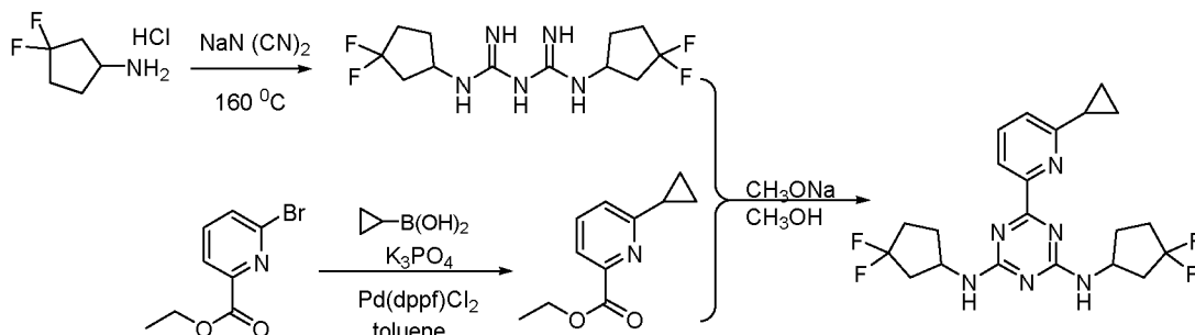
Scheme 19
