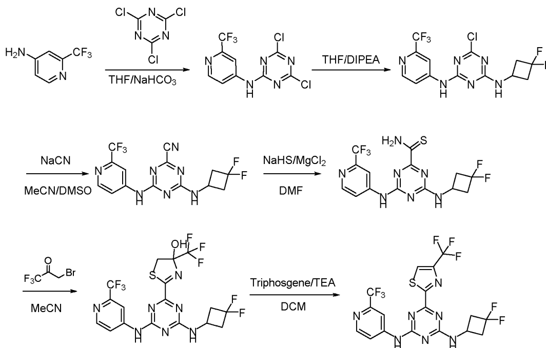
Scheme 37
