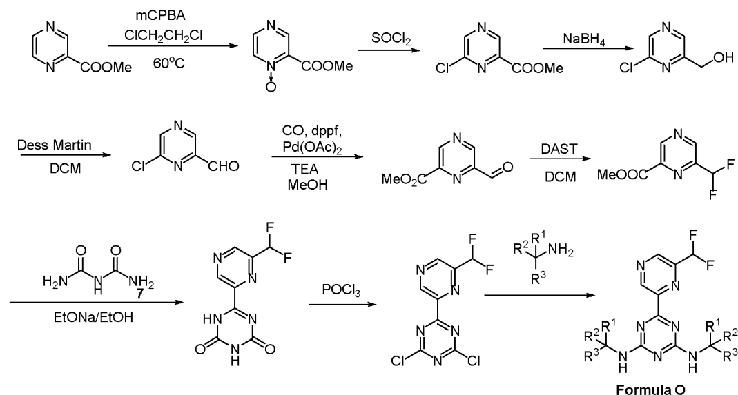
Scheme 22
