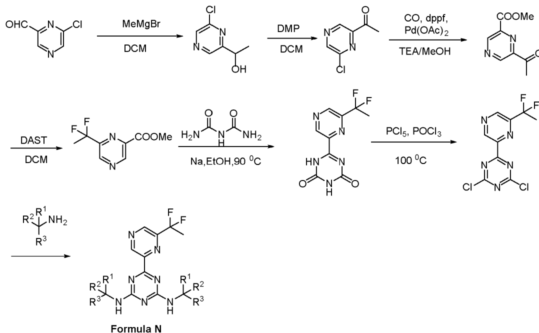
Scheme 21
