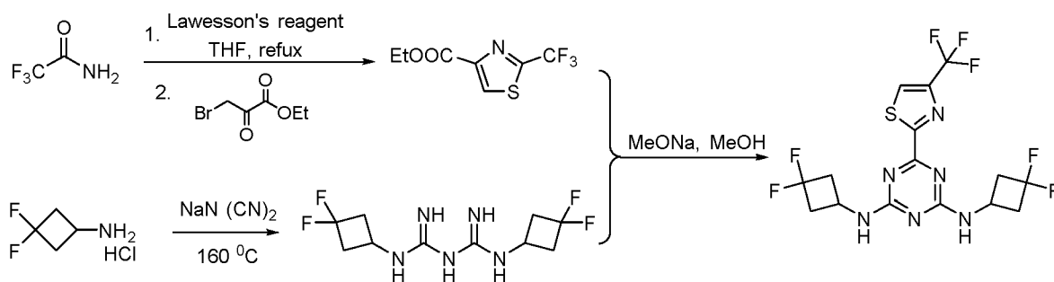
Scheme 25
