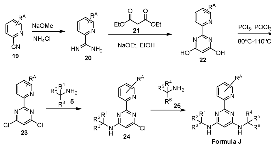
Scheme 7
