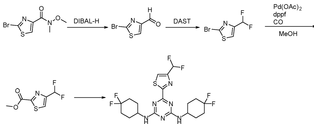
Scheme 27
