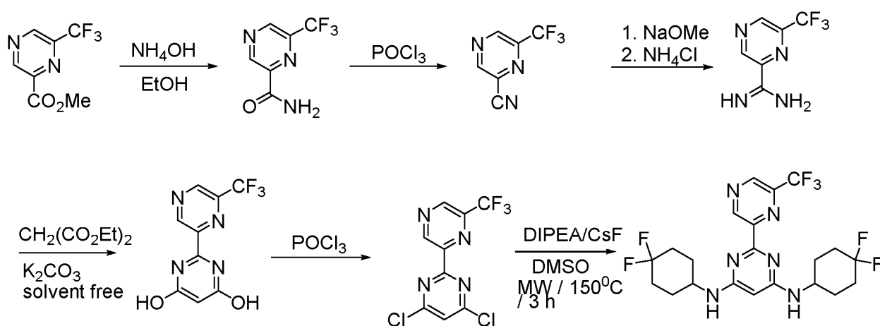
Scheme 35
