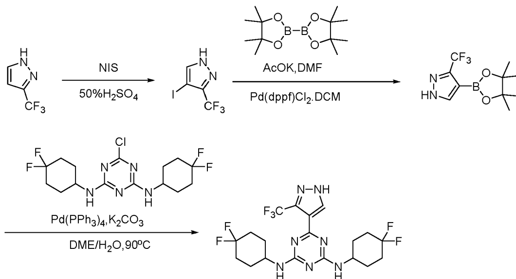
Scheme 31
