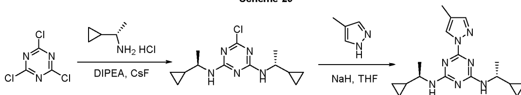
Scheme 29
