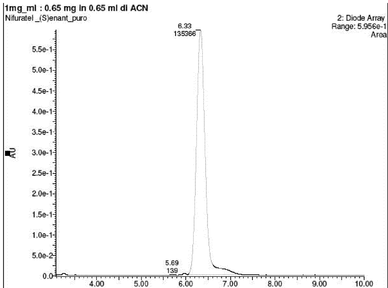
Figure 1b. Profile of s-nifuratel (Ib)
