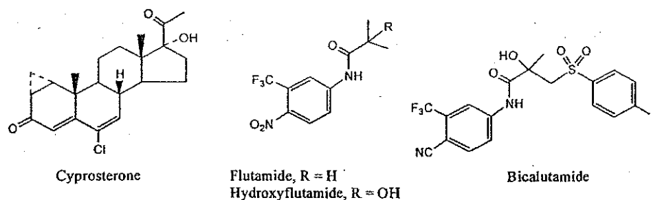
Chart 1. Structures of cyproterone, hydroxyflutamide, and bicalutamide.
