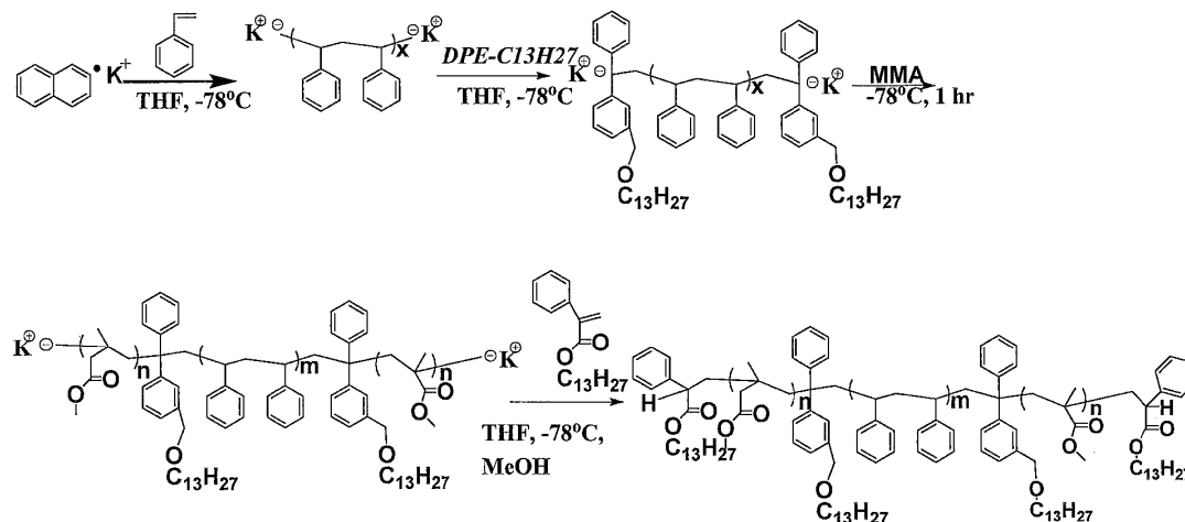
Scheme 1: Synthesis of ABA with non-polar tethered moieties
