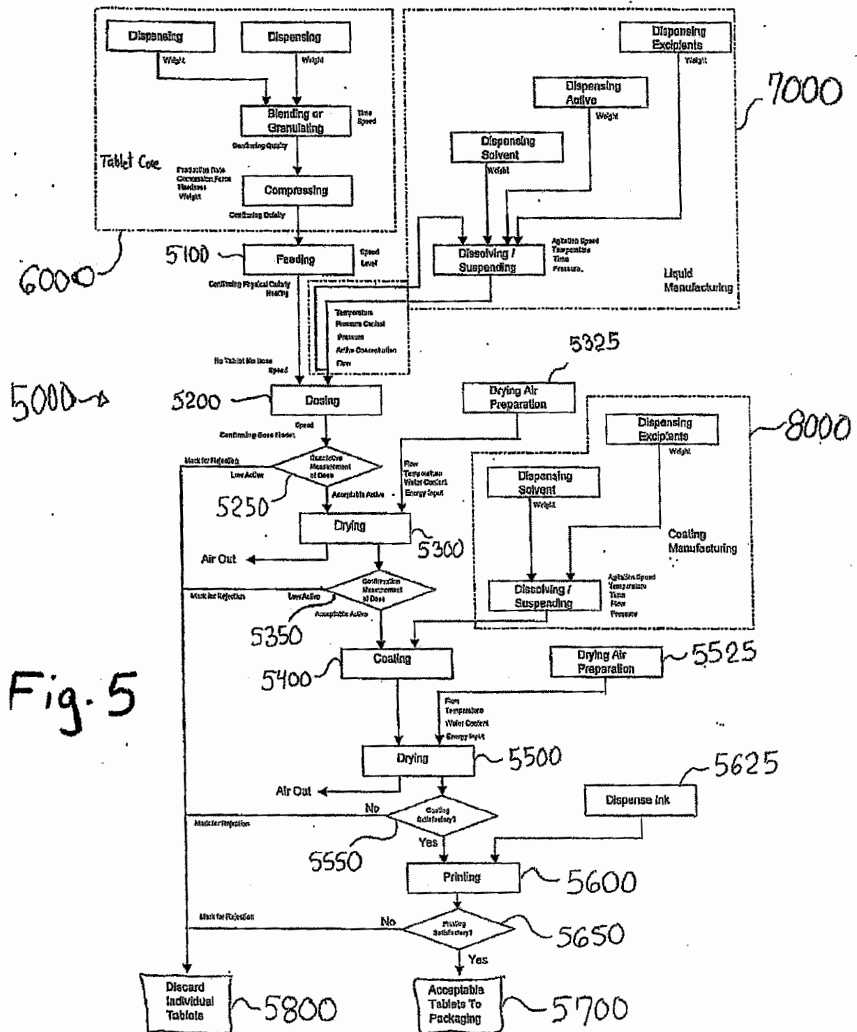
Liquid Dispensing Technology - Flow Diagram
