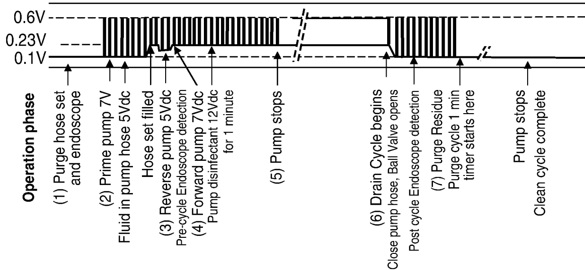
Typical waveform for 5 minute disinfection clean cycle with endoscope detection
