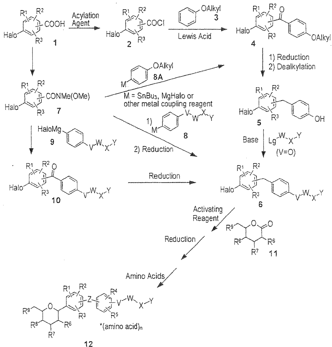
Scheme I
