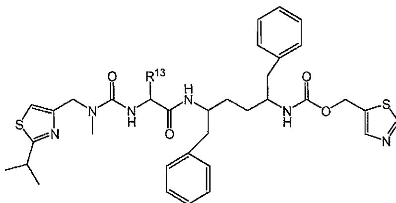
Formula IIC
