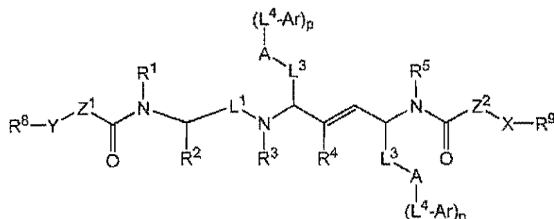
Formula IID
