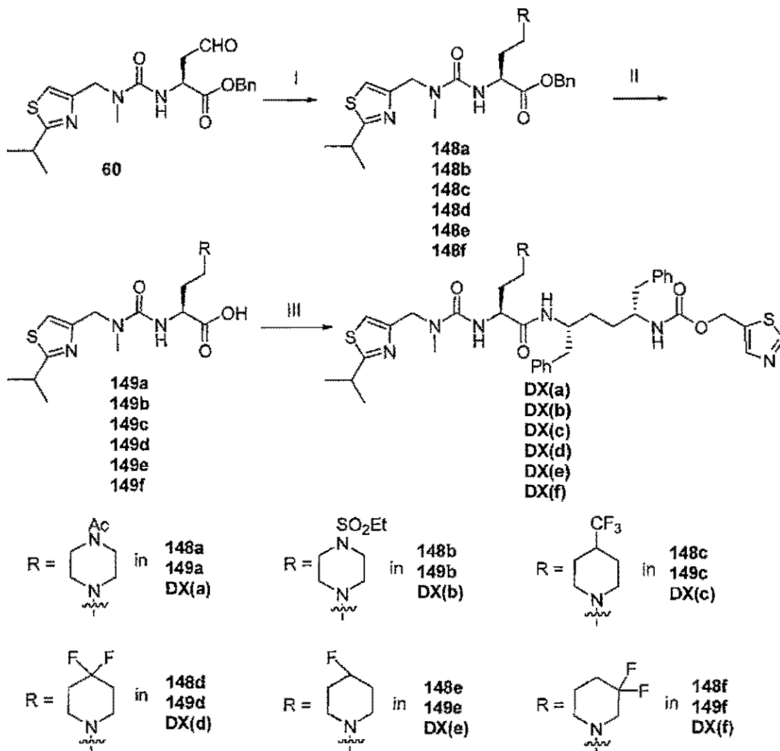
Scheme 99
