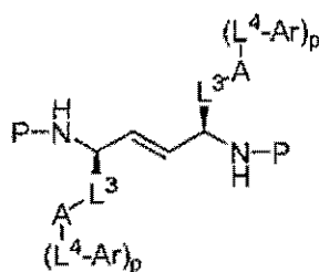
Analog of Compound 43; and
