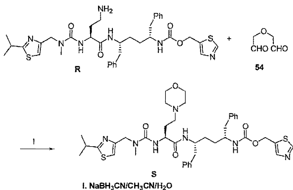
Scheme 21
