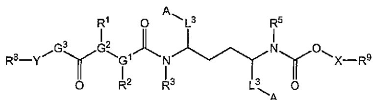
Formula IV
