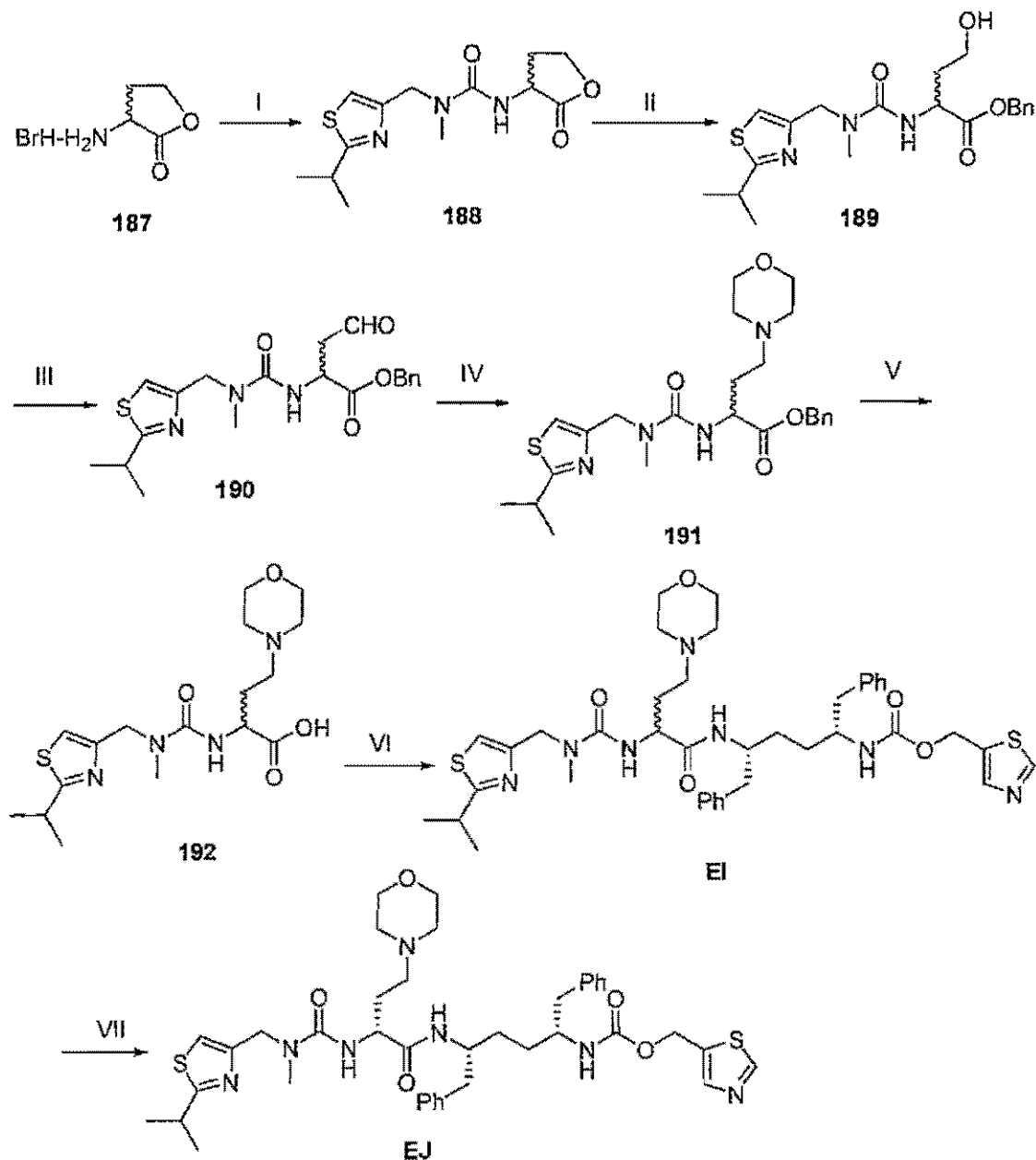
Scheme 110
