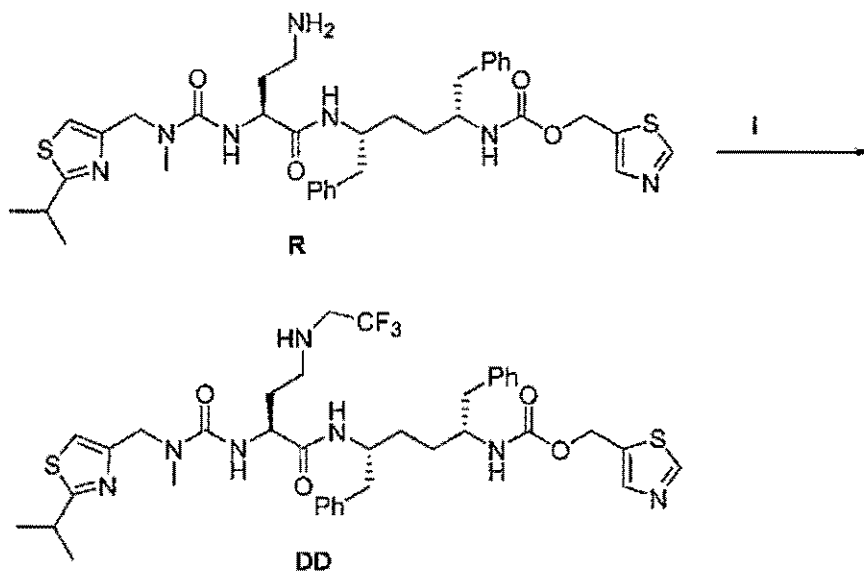
Scheme 85
