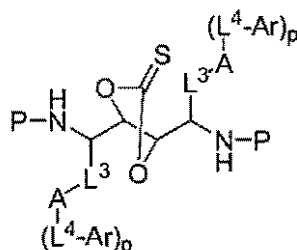
Analogs of Compound 26 ;
