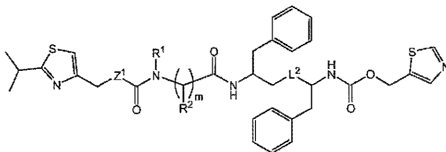
Formula IA.
