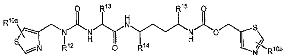
Formula IIB
