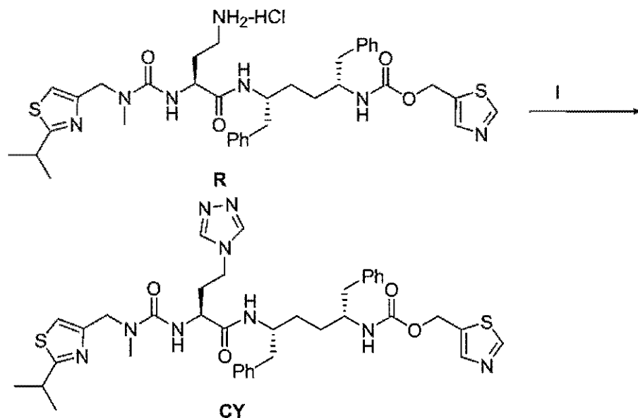
Scheme 80
