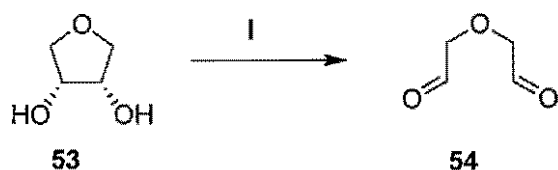
Scheme 20
