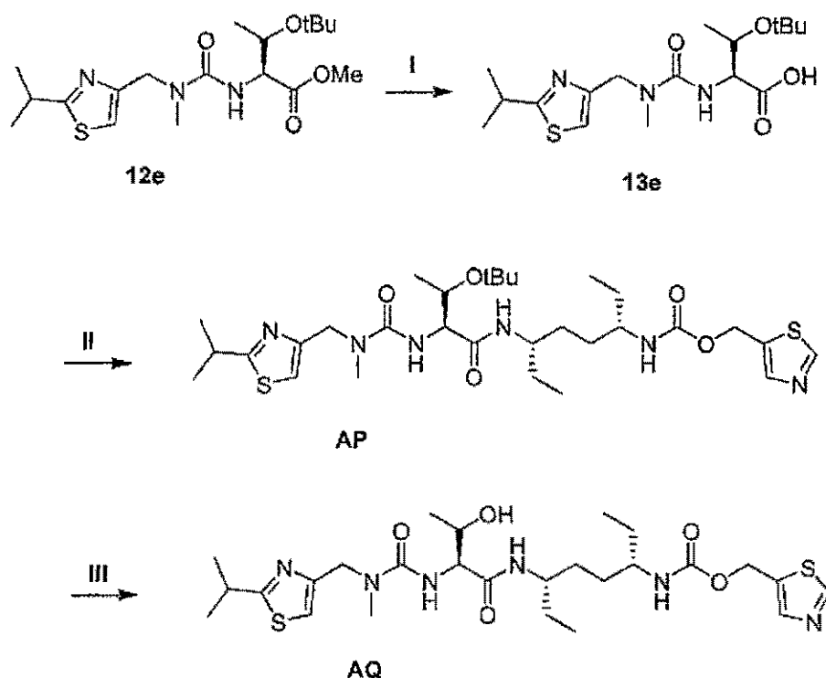
Scheme 34
