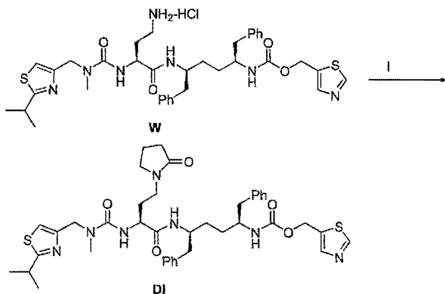
Scheme 89
