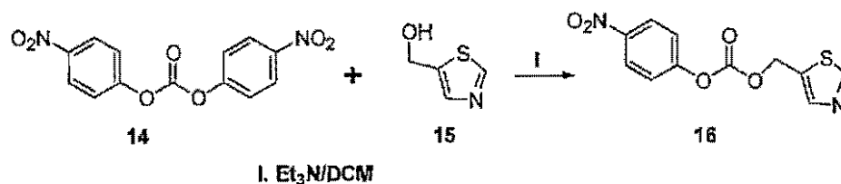
Scheme 7
