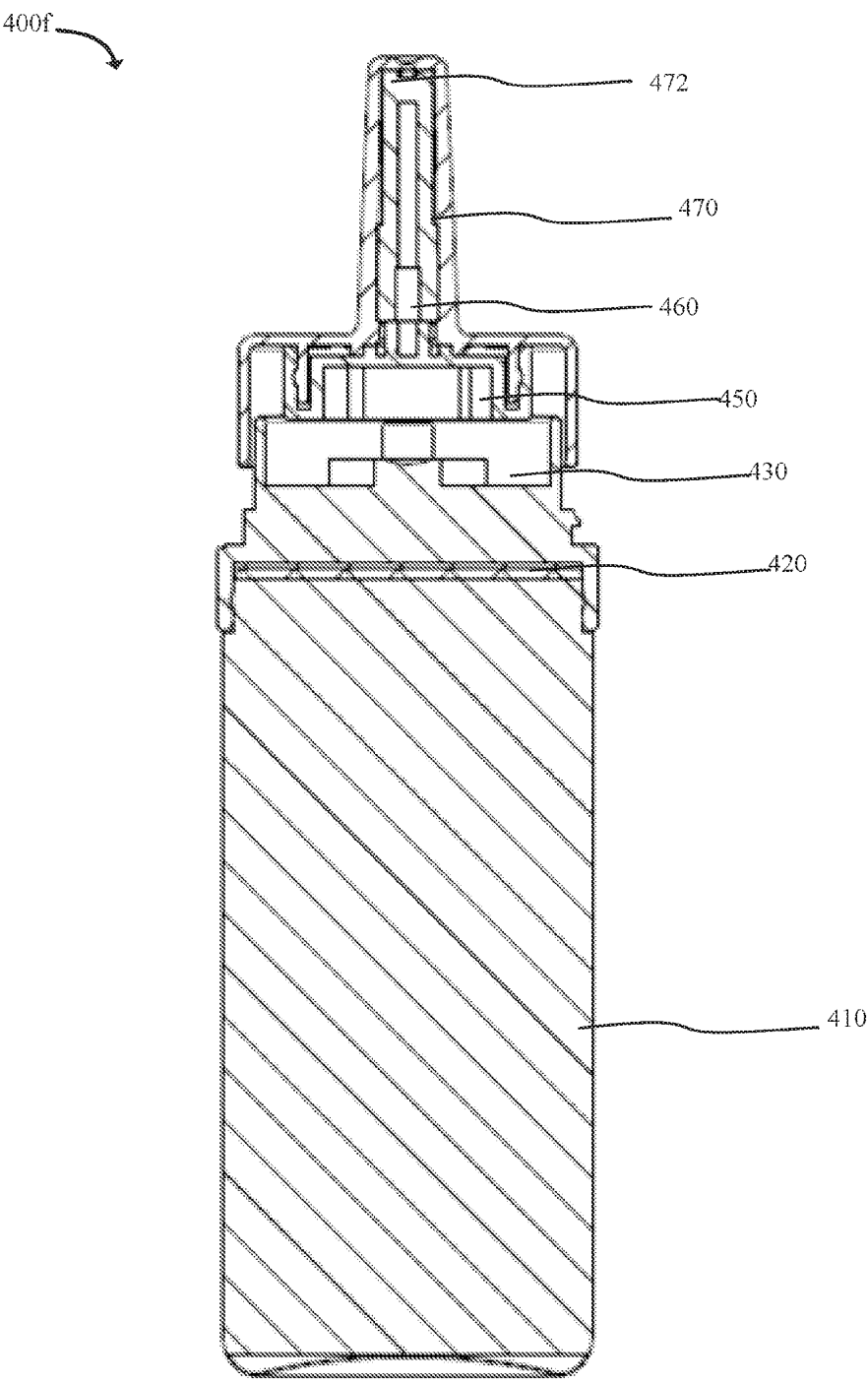
SECTION B-B
