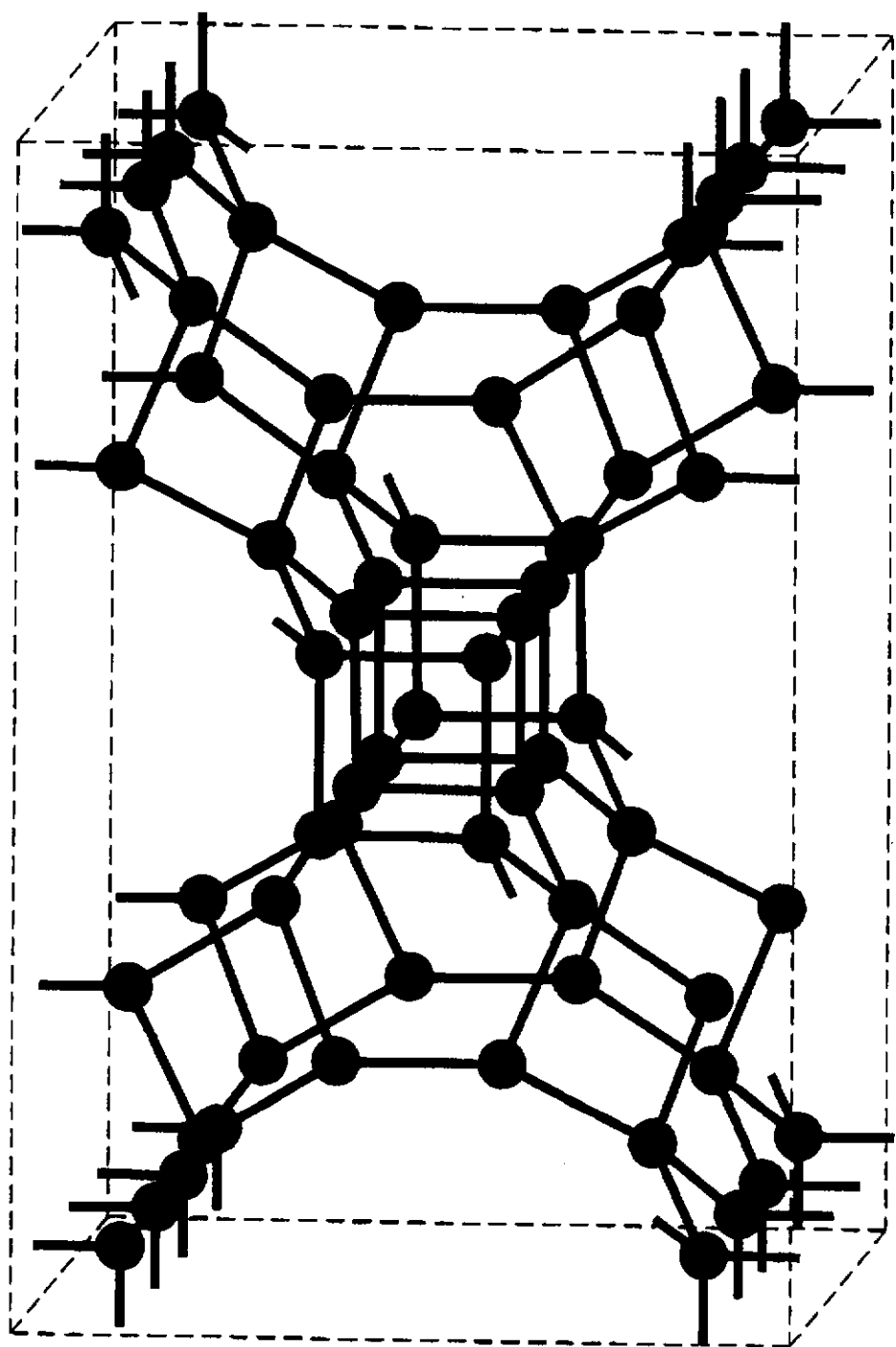
Unit cell of zeolite ITQ-24
