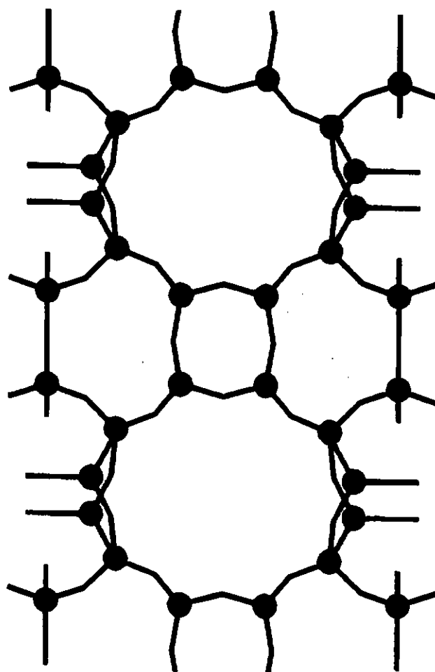
View of the channels formed by 10 tetrahedrons of zeolite ITQ-24
