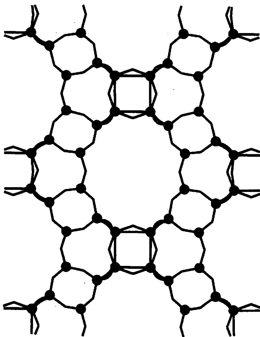
View of the rectilinear channels formed by 12 tetrahedrons of zeolite ITQ-24
