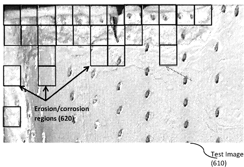
Figure 6B Erosion / corrosion detection results.
