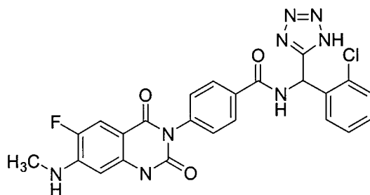
N-((3,4-dichlorophenyl)(1H-tetrazol-5-yl)methyl)-4-(6-fluoro-7-(methylamino)-2,4-dioxo-1,2-dihydroquinazolin-3(4H)-yl)benzamide (Compound 29);
