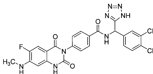
5 N-((3,5-dichlorophenyl)(1H-tetrazol-5-yl)methyl)-4-(6-fluoro-7-(methylamino)-2,4-dioxo-1,2-dihydroquinazolin-3(4H)-yl)benzamide (Compound 30);
