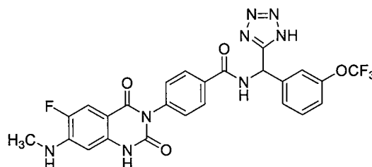
10 N-((1H-tetrazol-5-yl)(3-(trifluoromethyl)phenyl)methyl)-4-(6-fluoro-7-(methylamino)-2,4-dioxo-1,2-dihydroquinazolin-3(4H)-yl)benzamide (Compound 34)
