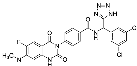
N-((1H-tetrazol-5-yl)(3-(trifluoromethoxy)phenyl)methyl)-4-(6-fluoro-7-(methylamino)-2,4-dioxo-1,2-dihydroquinazolin-3(4H)-yl)benzamide (Compound 31);
