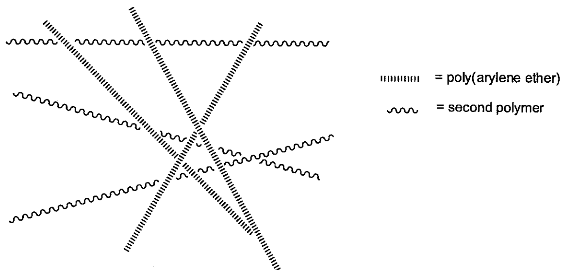
Figure 1. Semipenetrating Polymer Network with Poly(arylene ether)
