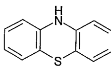
phenothiazine
