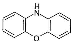
phenoxazine
