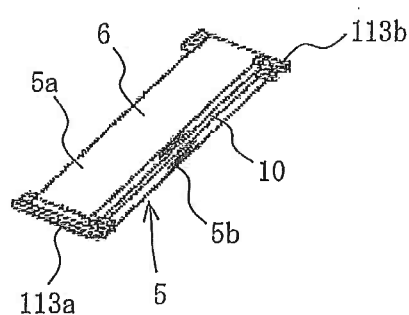
(g) CORE FORMATION STEP
