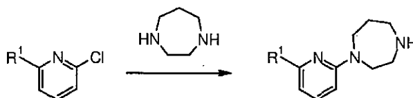
20 Table 7: Preparation of 6-(1,4-diazepan-1-yl)-2-substituted pyridine intermediates
