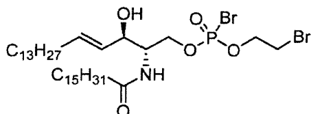
2-bromoethyl ((2S,3R,E)-3-hydroxy-2-palmitamido-octadec-4-en-1-yl) phosphorobromidate ;
