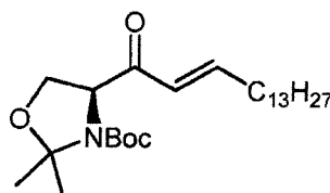
(S)-3-(tert-butoxycarbonyl)-4-(1-oxo-hexadec-2-enyl)-2,2-dimethyloxazolidin Compound Ie ;
