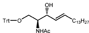
1-O-Trityl-D-erythro-ceramide Compound 1c-1
