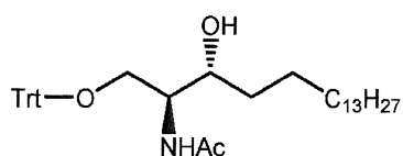
1-O-Trityl-D-erythro-dihydroceramide Compound VIIf -Trt ;
