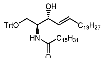
N-Palmitoyl-1-O-Trityl-D-erythro-sphingosine Compound 1h-1
