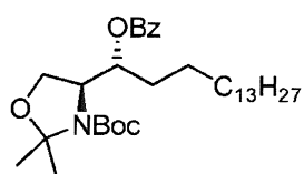
(S)-tert-butyl 4-((R)-1-(benzoyloxy)hexadecyl)-2,2-dimethyloxazolidine-3-carboxylate Compound XIa ;
