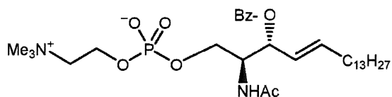
Compound 1g - Bz
