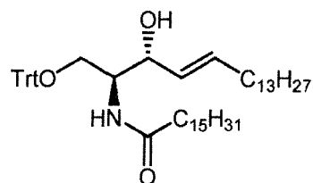
N-Palmitoyl-1-O-Trityl- D -erythro-sphingosine Compound VIa ;
