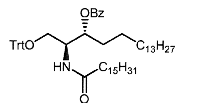
N-palmitoyl-1-O-Trityl-3-O-Benzoyl-D-erythro-dihydrosphingosine Compound VIIlb
