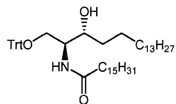
N-palmitoyl 1-O-Trityl-D-erythro-dihydrosphingosine Compound VIIla
