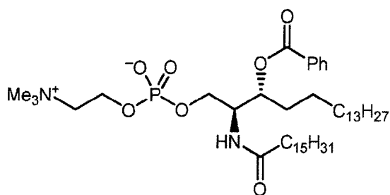
N-Palmitoyl-3-O-Benzoyl- D -erythro- dihydrosphingomyelin Compound VIIle ;
