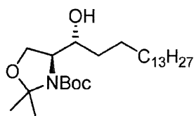
((S)-tert-butyl 4-((R)-1-hydroxyhexadecyl)-2,2-dimethyloxazolidine-3-carboxylate Compound 1la
