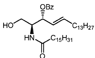
N-Palmitoyl-3-O-Benzoyl- D-erythro-sphingosine Compound VIc ;
