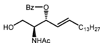
1-O-Benzoyl-D-erythro-ceramide Compound 1e-1
