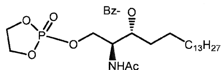
3-O-Benzoyl-D-erythro-1-O- (2-oxo-1,3,2-dioxaphospholan)-dihydroceramide Compound VIIf ;
