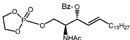
3-O-Benzoyl-D-erythro-1-O-(2-oxo-1,3,2-dioxaphospholan)-ceramide Compound 1f-1
