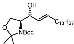
(2S,3R,4E)-3-(tert-butoxycarbonyl)-4-(1-hydroxyhexadec-2-enyl)-2,2-dimethyloxazolidin Compound 1f
