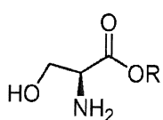
L-Serine Ester Compound Ia
