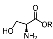
L-Serine Ester Compound Ia, and salts thereof;
