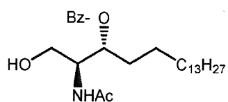
3-O-Benzoyl-D-erythro-dihydroceramide Compound VIIf ;
