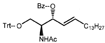
1-O-Benzoyl-3-O-Trityl-D-erythro-ceramide Compound 1d-1
