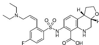
Mixture of cis enantiomers
