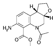
Mixture of cis enantiomers
