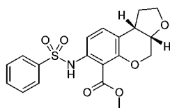
Mixture of cis enantiomers
