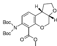
Mixture of cis enantiomers
