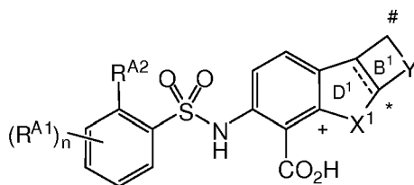
Formula III;
