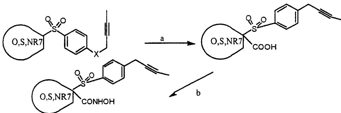
SCHEME:5
