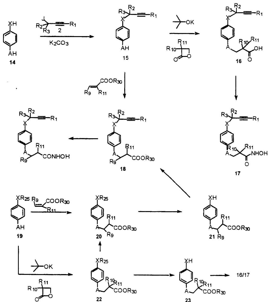
Scheme 8:
