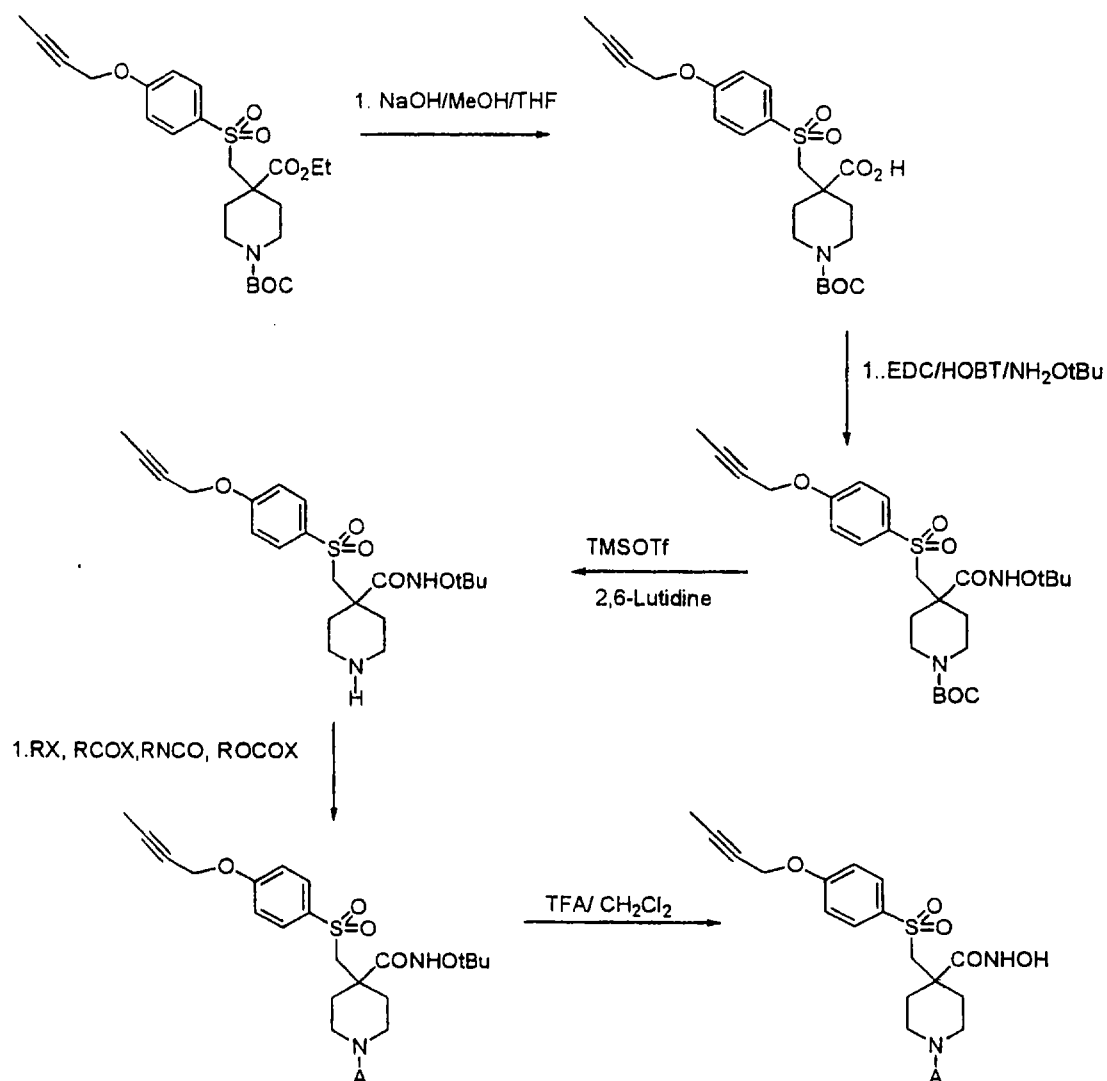
Scheme 16
