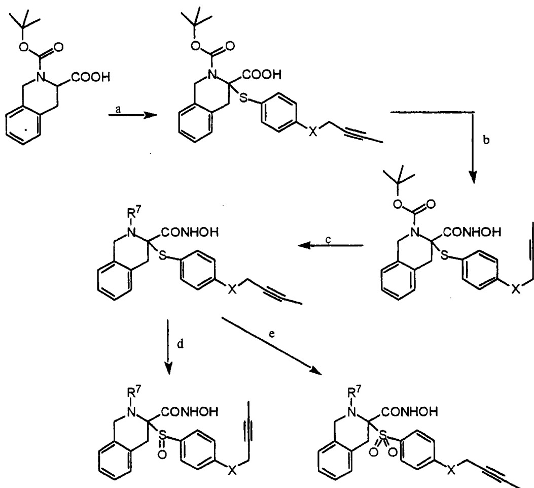
SCHEME:4
