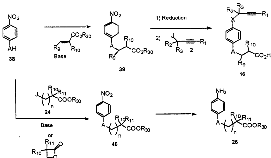
SCHEME 12
