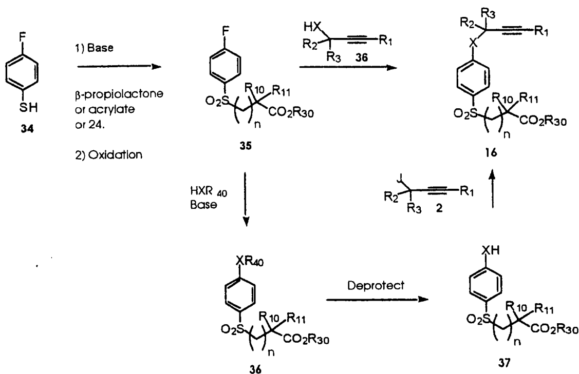
SCHEME 11
