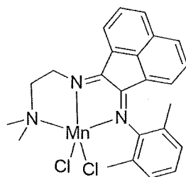
Structure XXII
