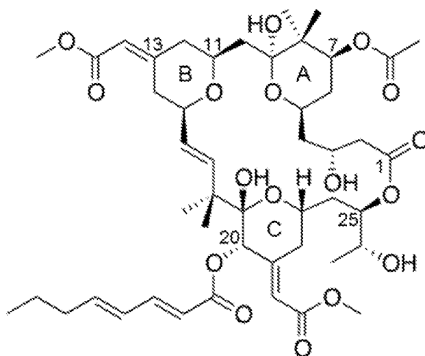
Bryostatin 1
