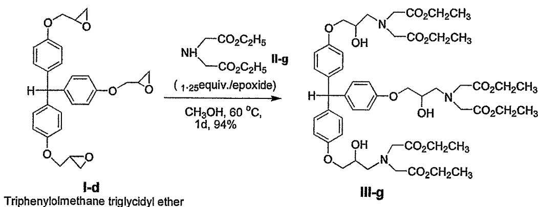
Scheme 22
