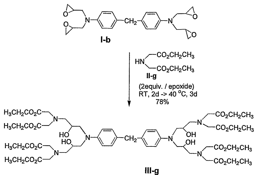
Scheme 29
