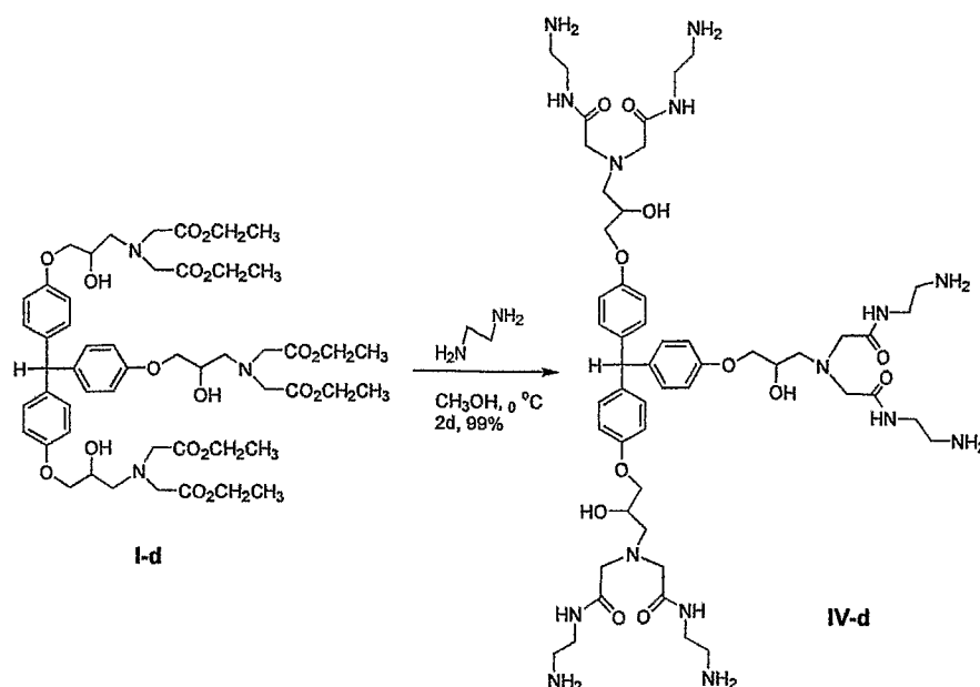
Scheme 23
