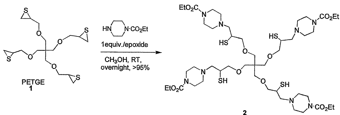
Scheme 33
