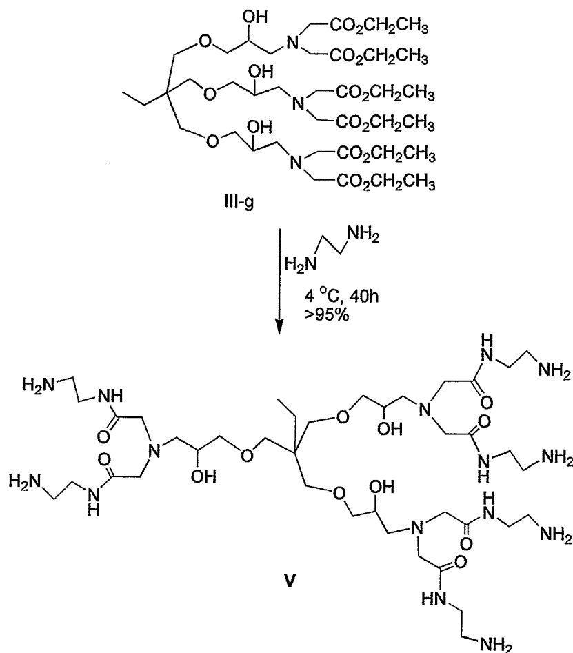
Scheme 7
