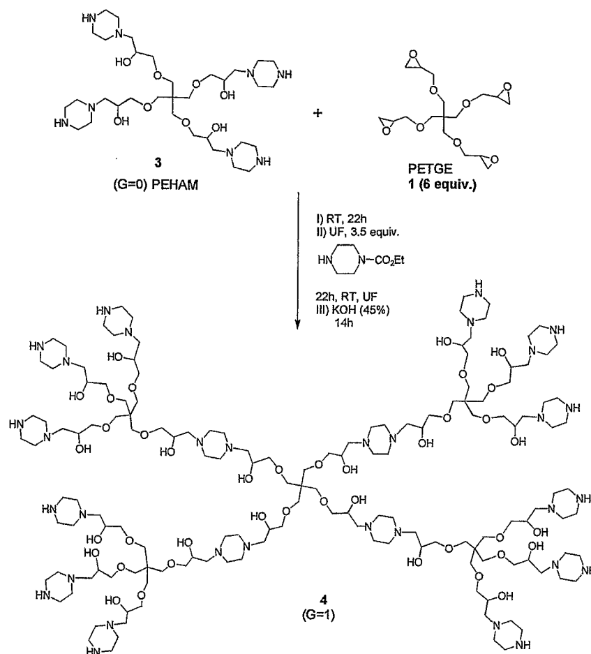
Scheme 12
