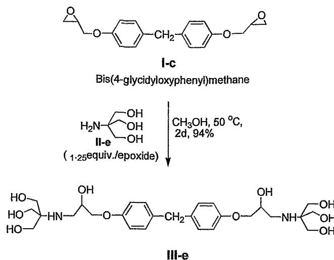
Scheme 24
