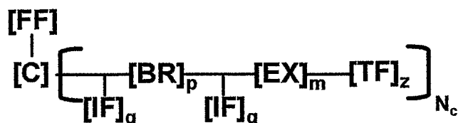
Formula (I)
