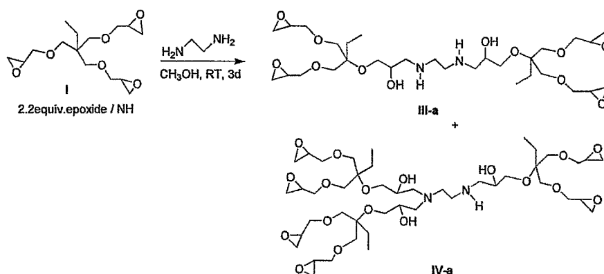
Scheme 37
