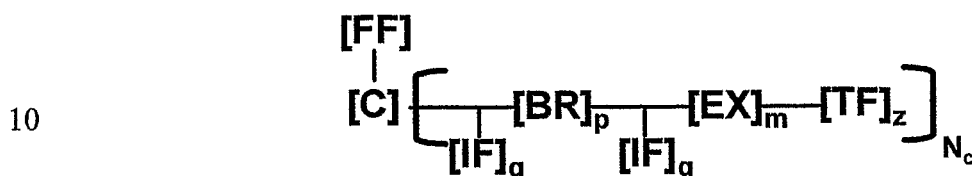
Formula (I)
