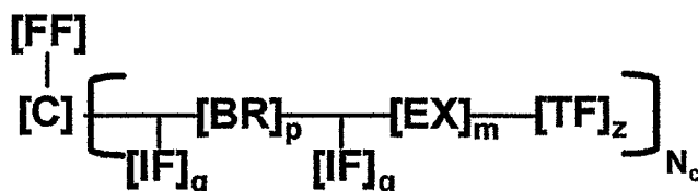
Formula (I)
