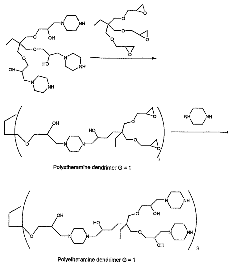
Scheme 4
