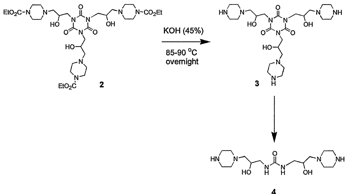
Scheme 35
