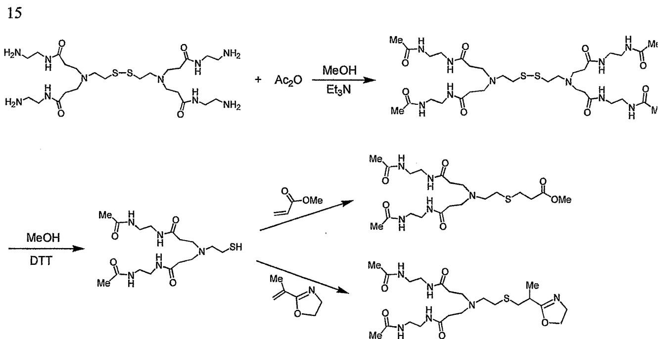
Scheme 40
