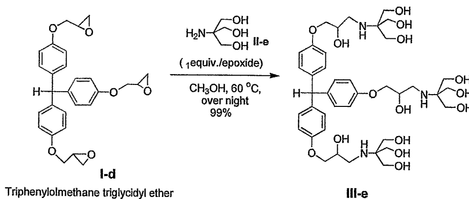
Scheme 20
