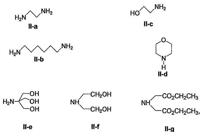
Branch cell reagents; Figure-2
