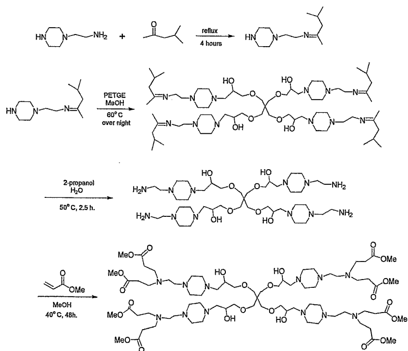
Scheme 17
