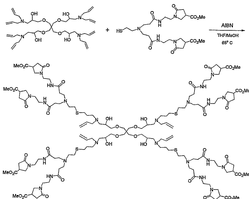
Scheme 39
