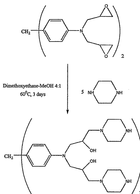
Scheme 31
