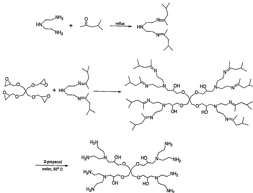
Scheme 14
