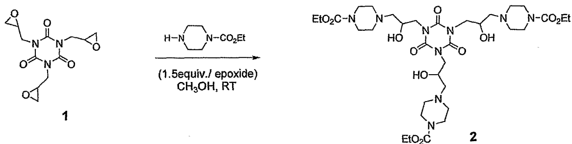
Scheme 34
