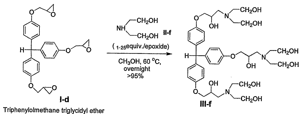
Scheme 21
