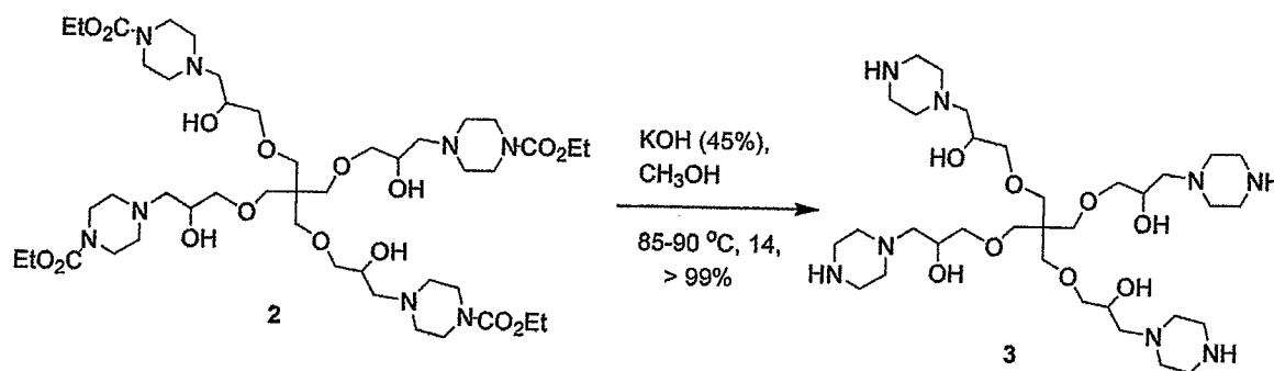
Scheme 11
