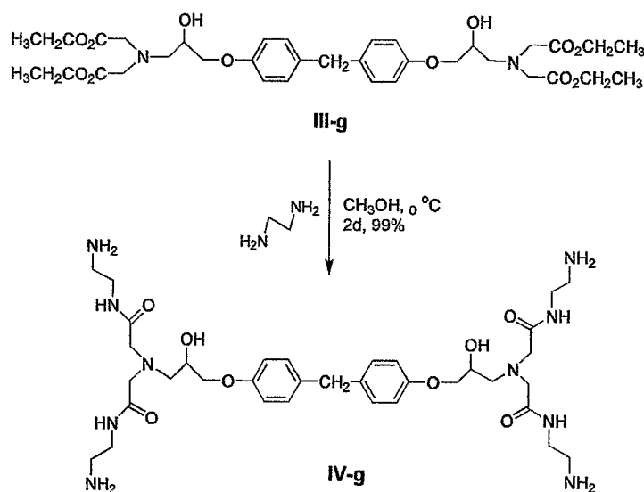
Scheme 26
