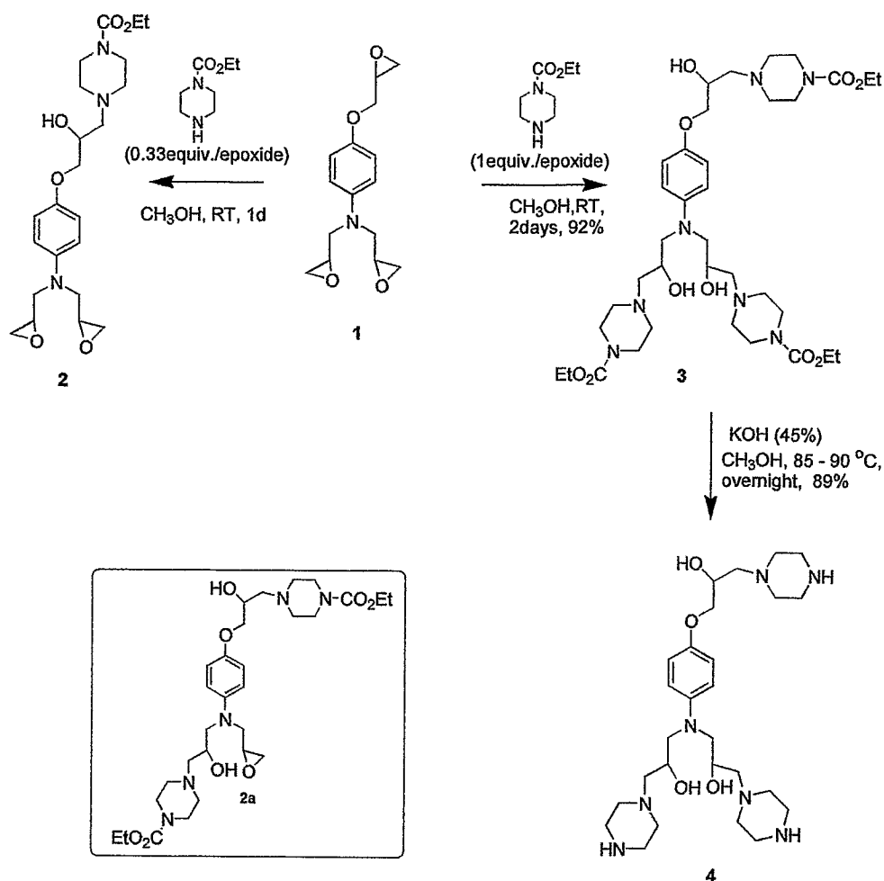
Scheme 32
