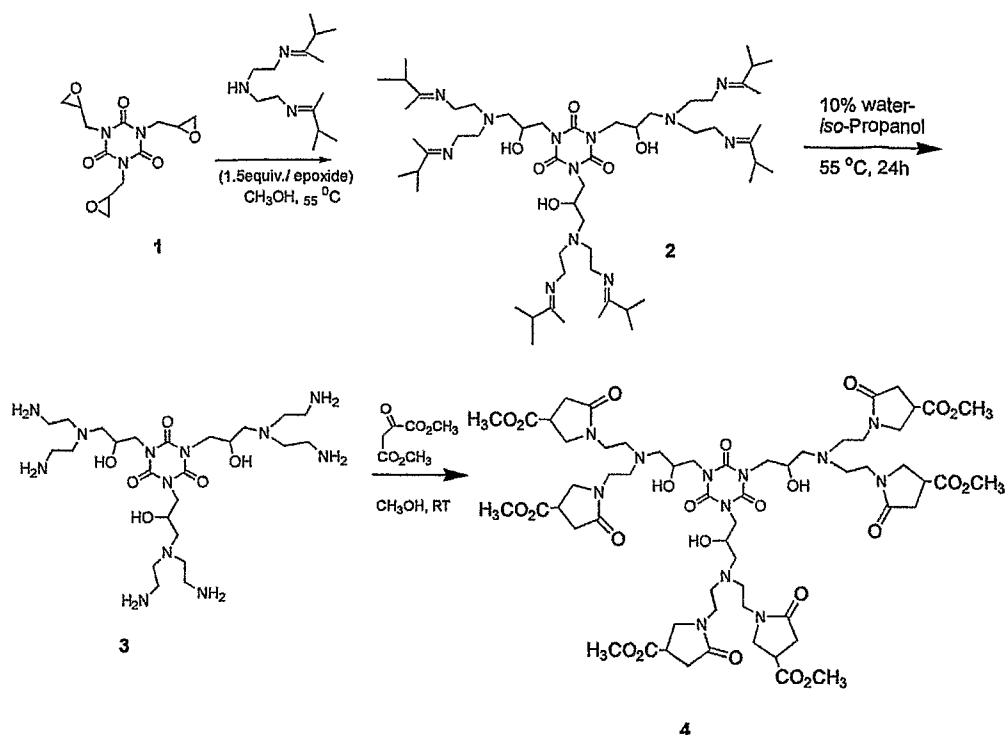
Scheme 36
