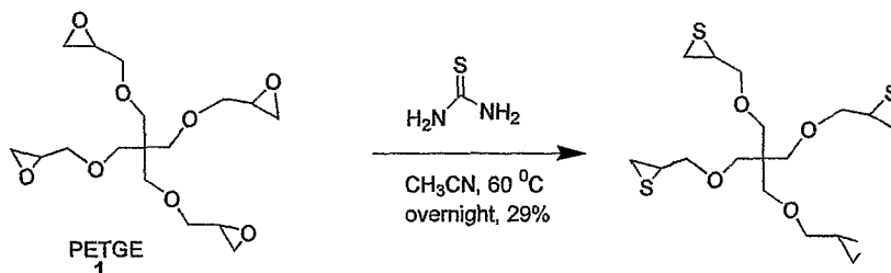
Scheme B
