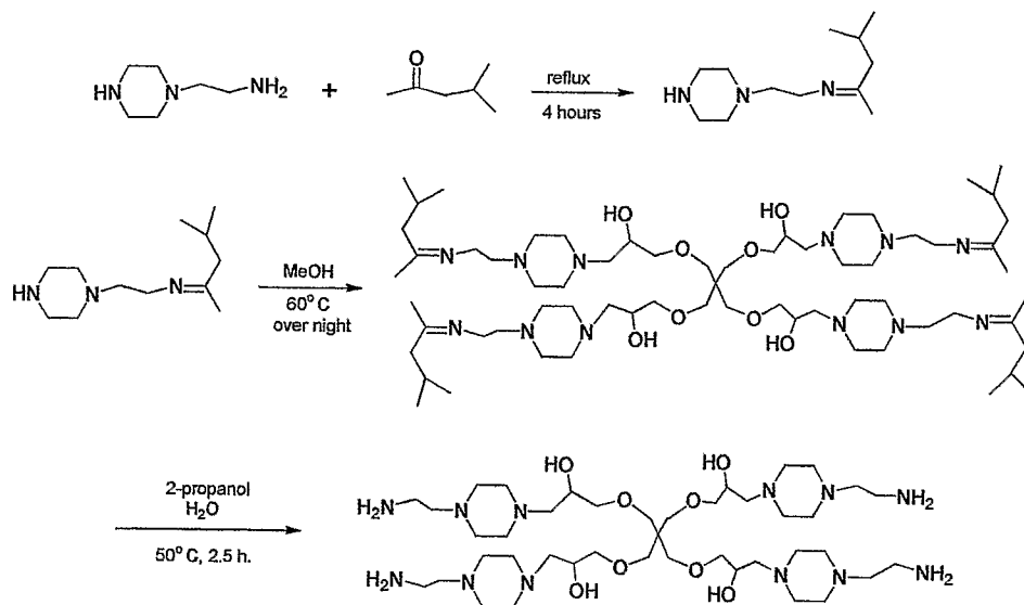
Scheme 13
