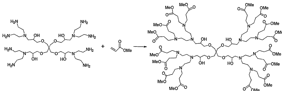
Scheme 18
