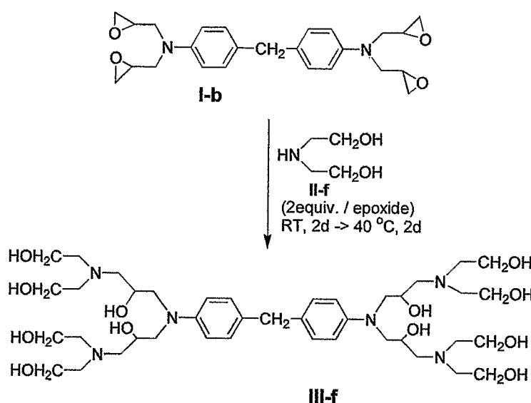
Scheme 27
