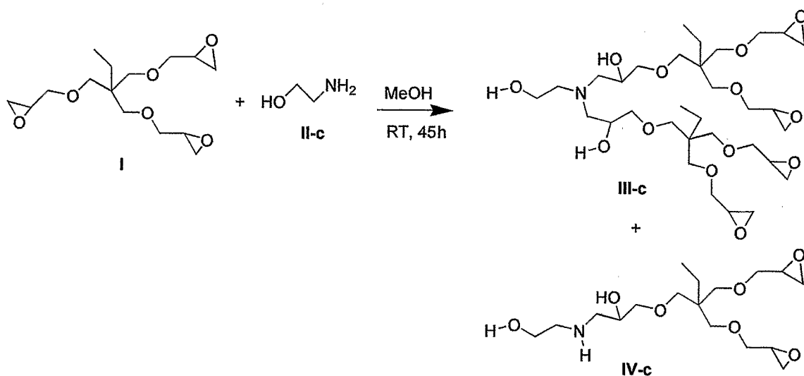
Scheme 38
