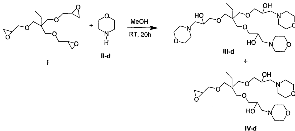
Scheme 9
