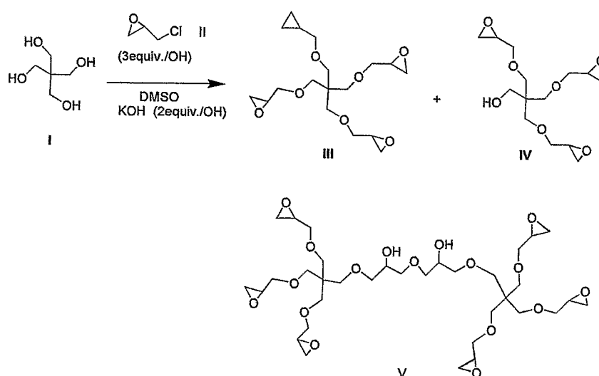
Scheme A
