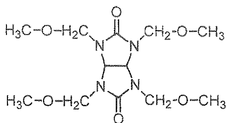
NIKALAC MX-270
