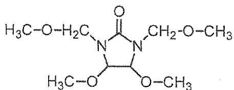
NIKALAC MX-280
