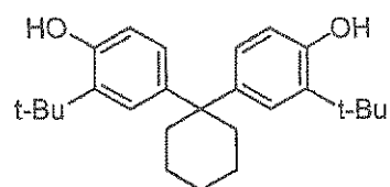
Bis0 TBP-Z
