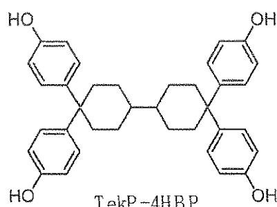
Bis0 TBP-Z
