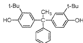
BisOTBP-AP
