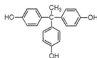
TrisP-HAP
