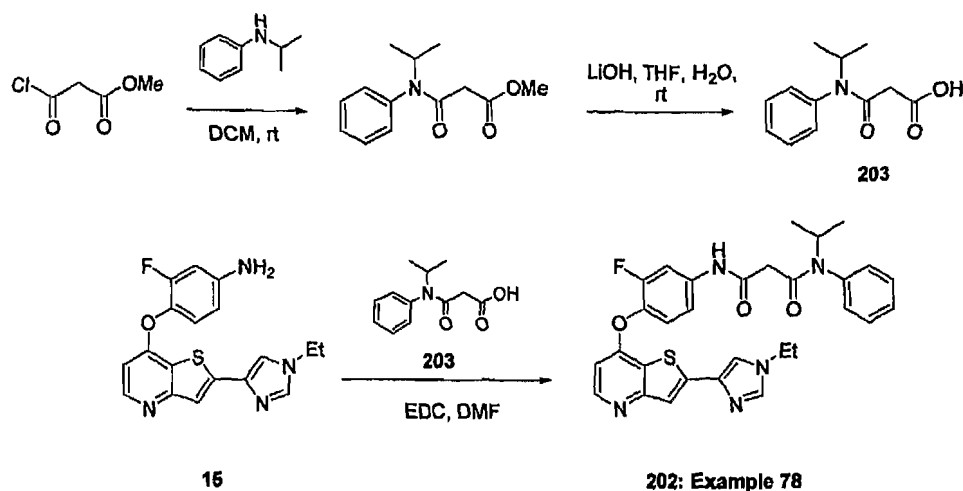
Scheme 57
