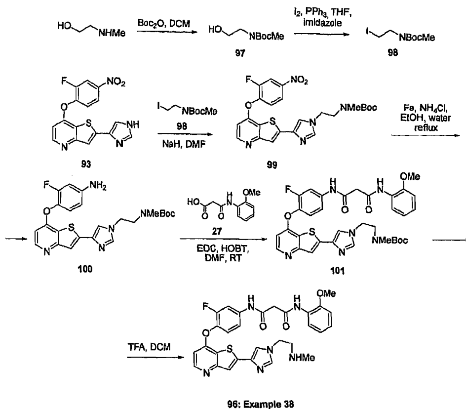
Scheme 30
