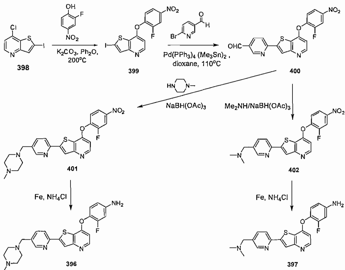
Scheme 87
