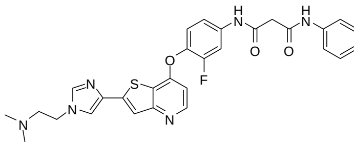
N -(4-(2-(1-(2-(dimethylamino)ethyl)-1 H -imidazol-4-yl)thieno[3,2- b ]pyridin-7-yloxy)-3-fluorophenyl)- N -phenylcyclopropane-1,1-dicarboxamide,
