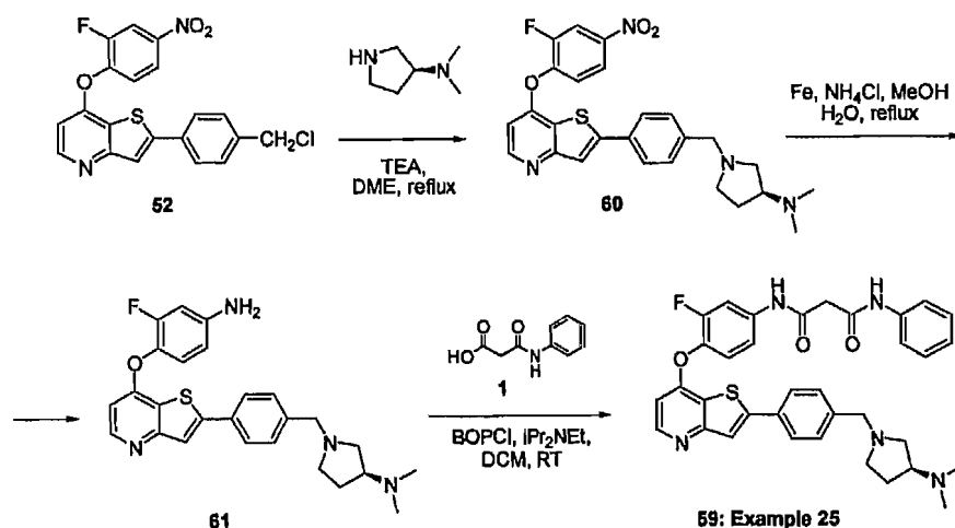
Scheme 21
