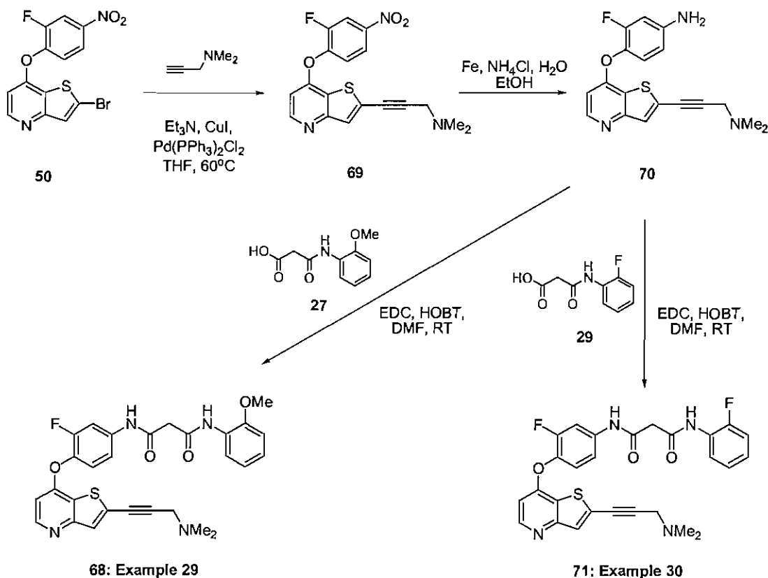
Scheme 24
