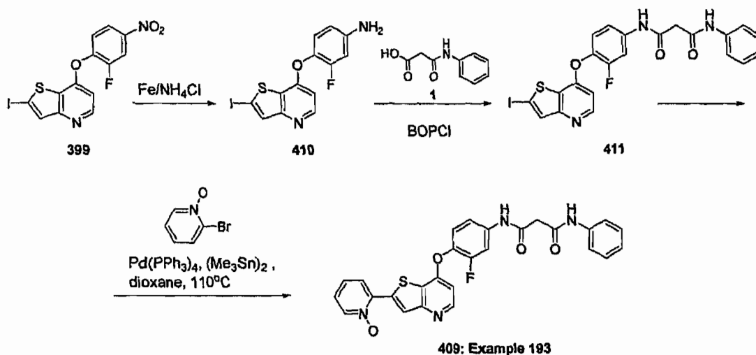
Scheme 89
