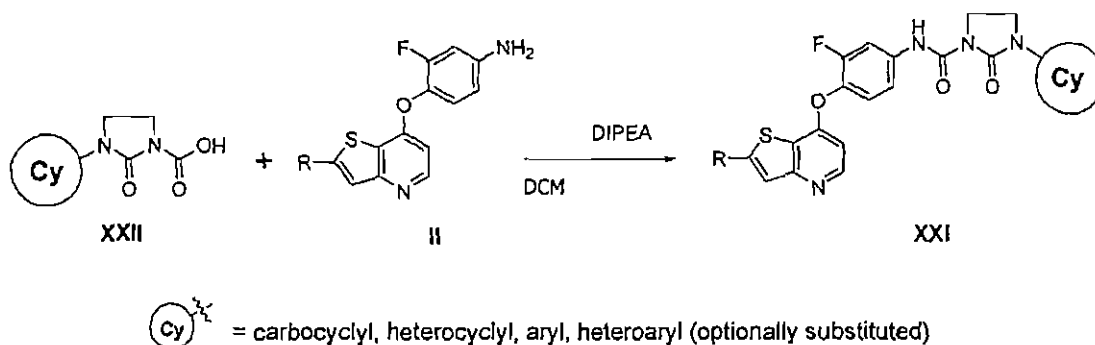
Scheme G
