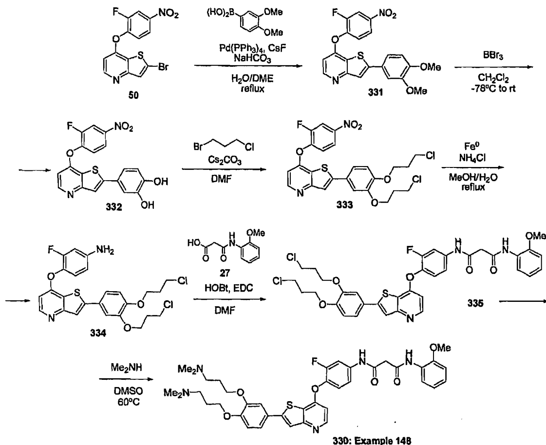
Scheme 77
