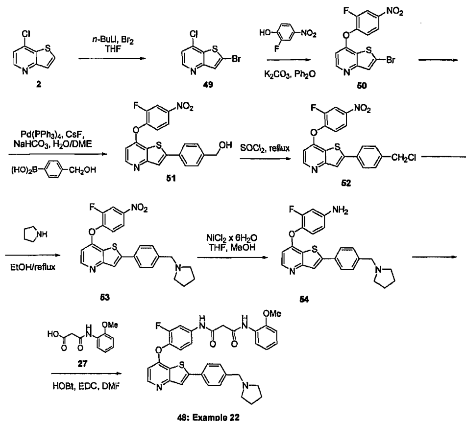
Scheme 18
