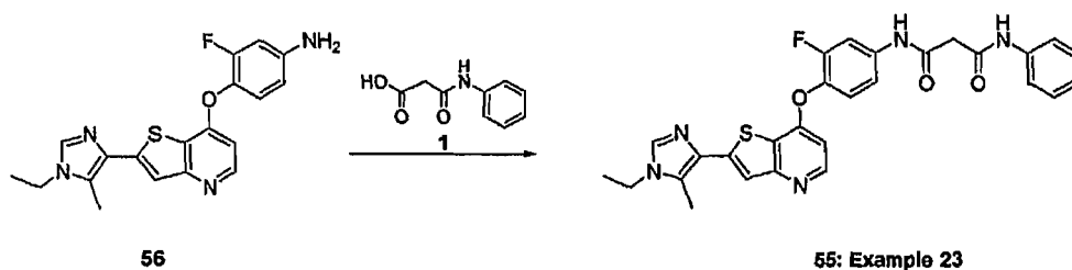
Scheme 19
