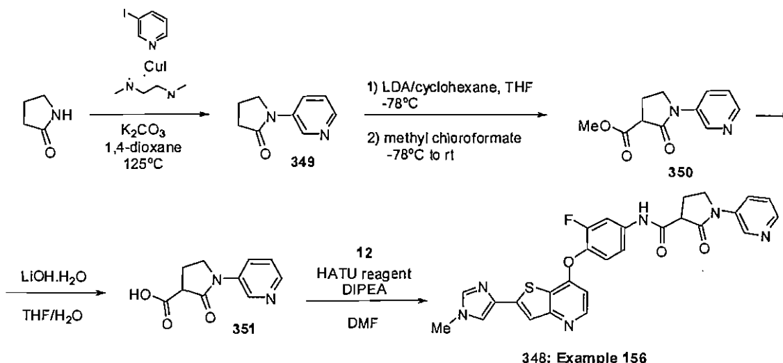
Scheme 80
