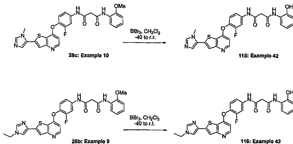
Scheme 34
