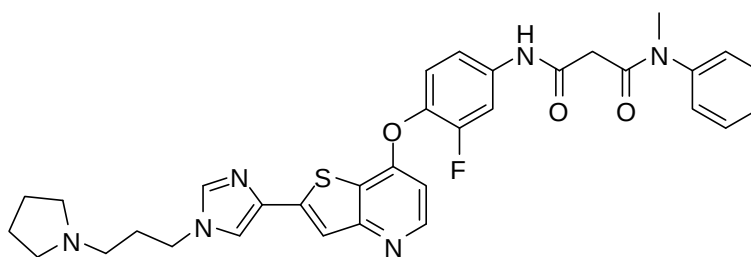
N 1 -(3-fluoro-4-(2-(1-(3-(pyrrolidin-1-yl)propyl)-1 H -imidazol-4-yl)thieno[3,2- b ]pyridin-7-yloxy)phenyl)- N 3 -methyl- N 3 -phenylmalonamide,
