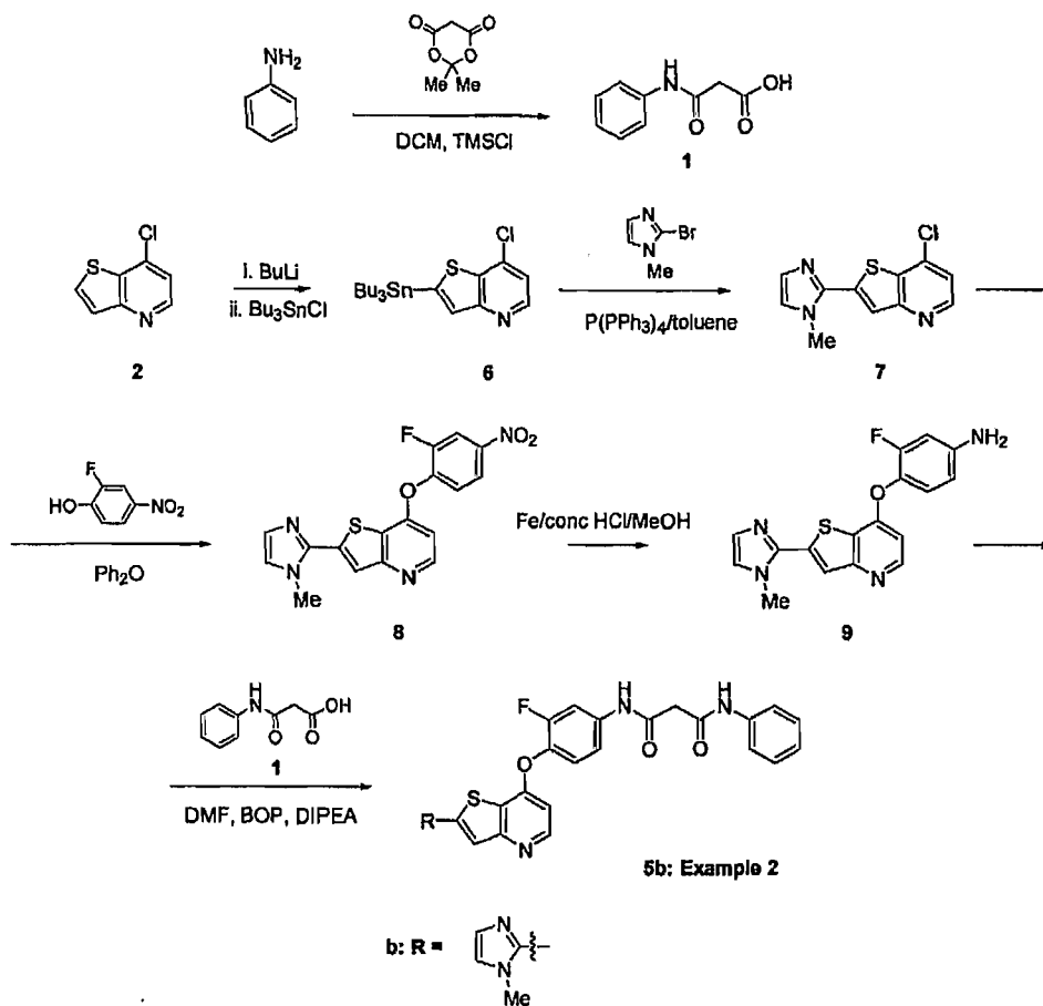
Scheme 2
