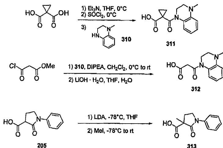
Scheme 74
