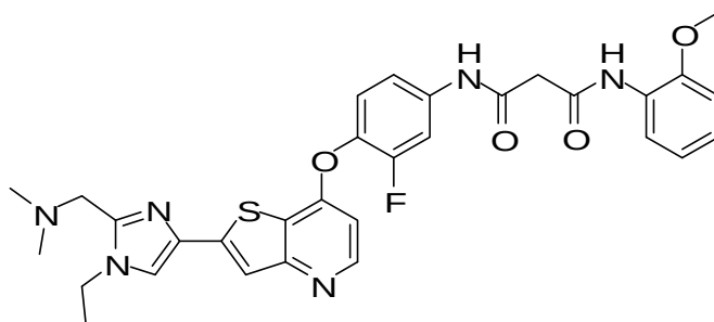
N 1 -(4-(2-(2-((Dimethylamino)methyl)-1-ethyl-1 H -imidazol-4-yl)thieno[3,2- b ]pyridin-7-yloxy)-3-fluorophenyl)- N 3 -(2-methoxyphenyl)malonamide,
