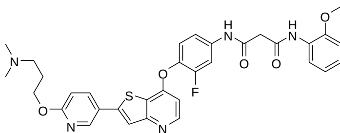
N^1 -(3-Fluoro-4-(2-(5-((4-methylpiperazin-1-yl)methyl)pyridin-2-yl)thieno[3,2-b]pyridin-7-yloxy)phenyl)- N^3 -phenylmalonamide
