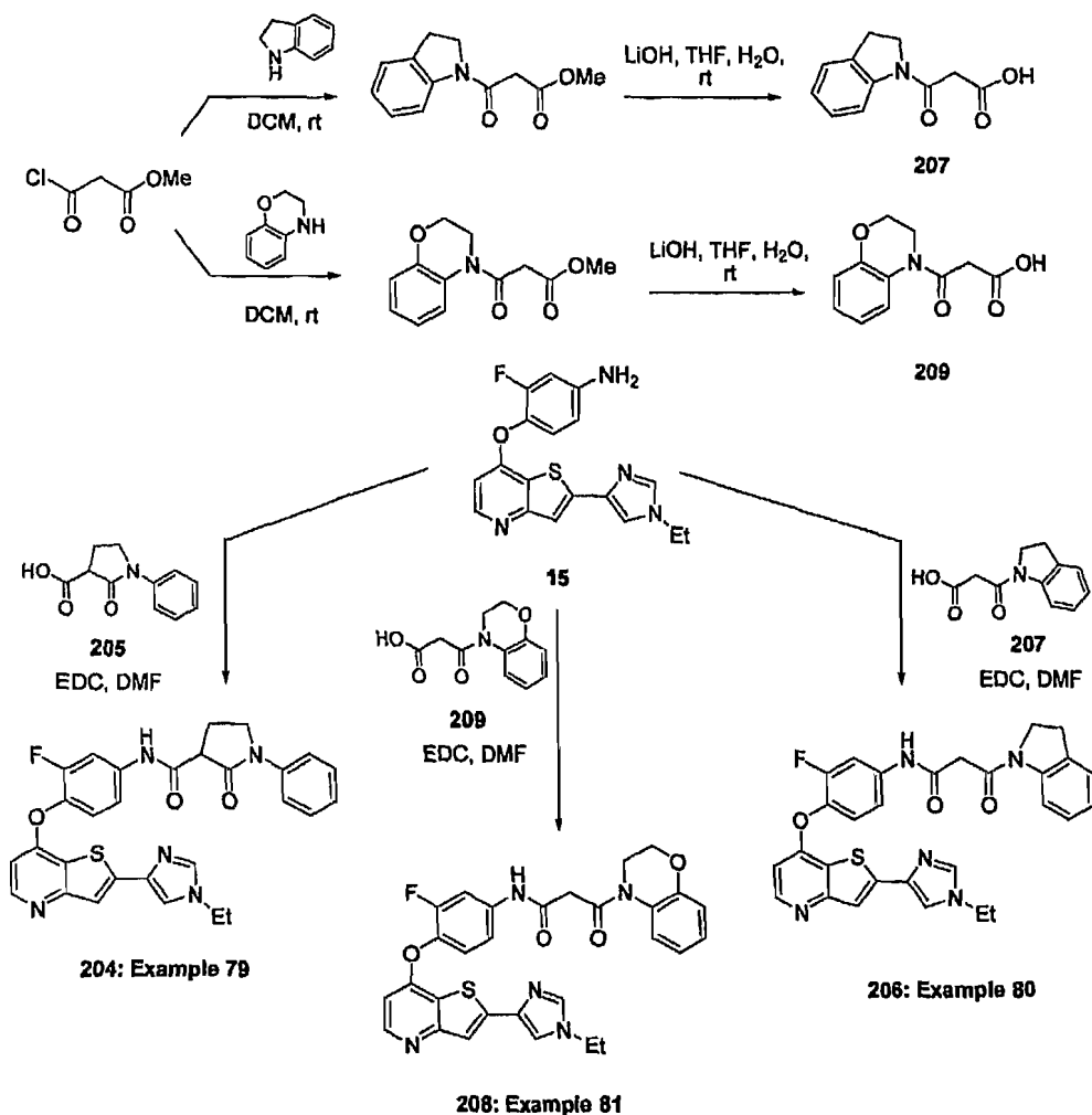
Scheme 58
