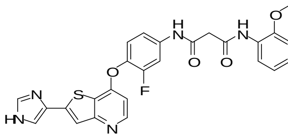
N 1 -(4-(2-(1-ethyl-2-methyl-1 H -imidazol-4-yl)thieno[3,2- b ]pyridin-7-yloxy)-3-fluorophenyl)- N 3 -(2-methoxyphenyl)malonamide,
