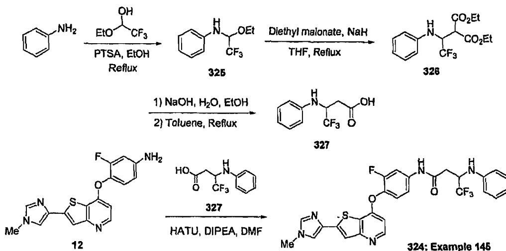
Scheme 76
