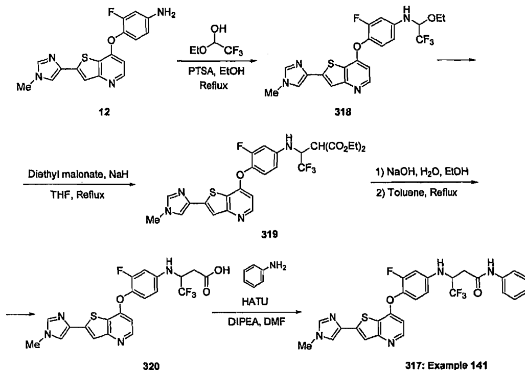
Scheme 75
