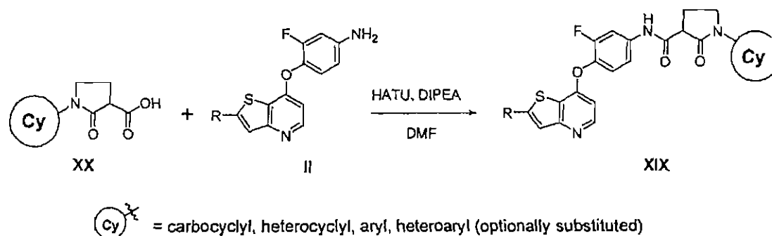
Scheme F
