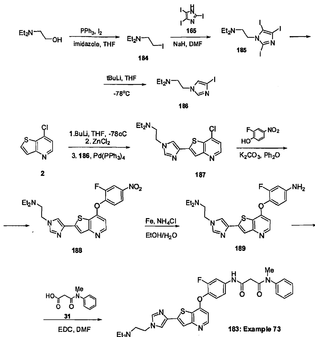
Scheme 52
