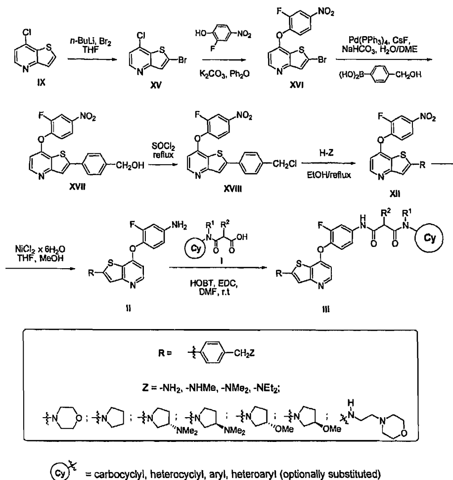
Scheme E
