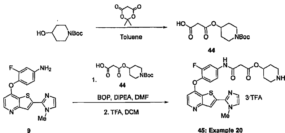
Scheme 16
