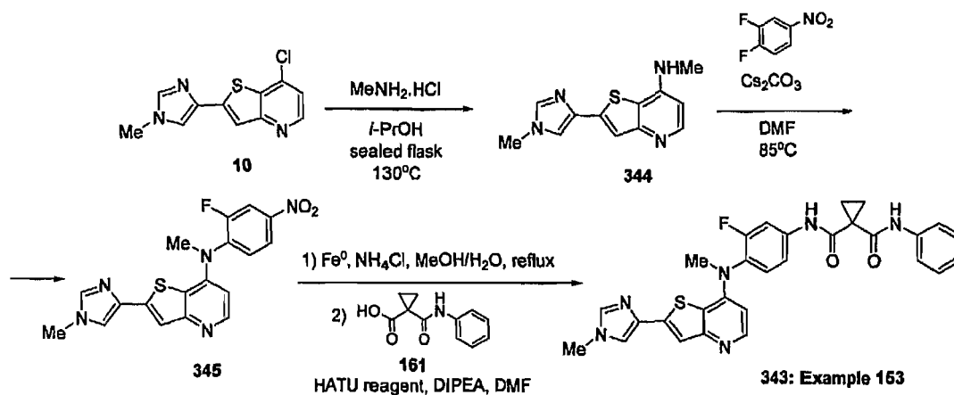
Scheme 79
