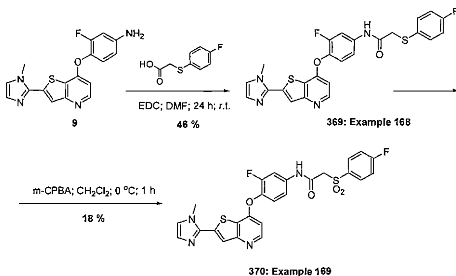
Scheme 83
