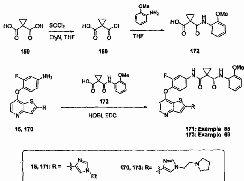
Scheme 47
