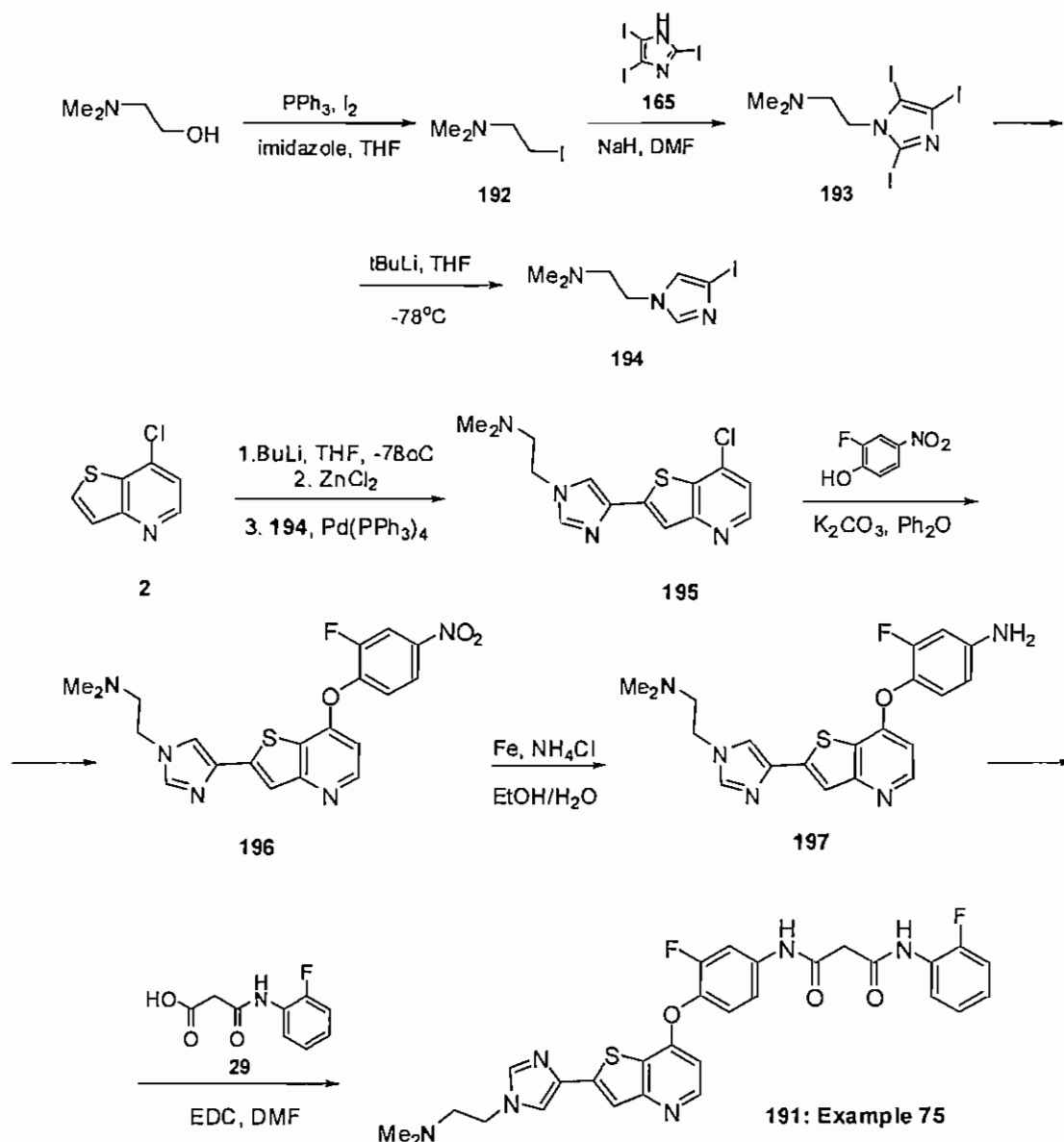
Scheme 54
