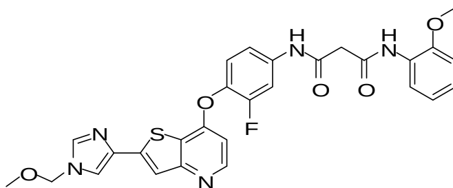
N 1 -(3-Fluoro-4-(2-(1-(2-(methylamino)ethyl)-1 H -imidazol-4-yl)thieno[3,2- b ]pyridin-7-yloxy)phenyl)- N 3 -(2-methoxyphenyl)malonamide,
