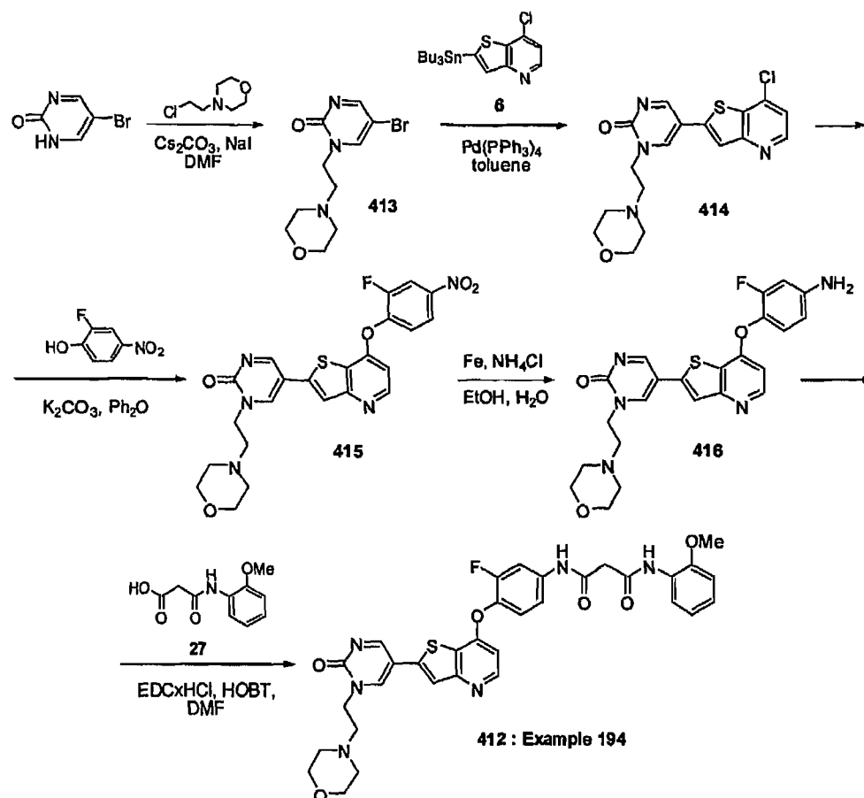
Scheme 90
