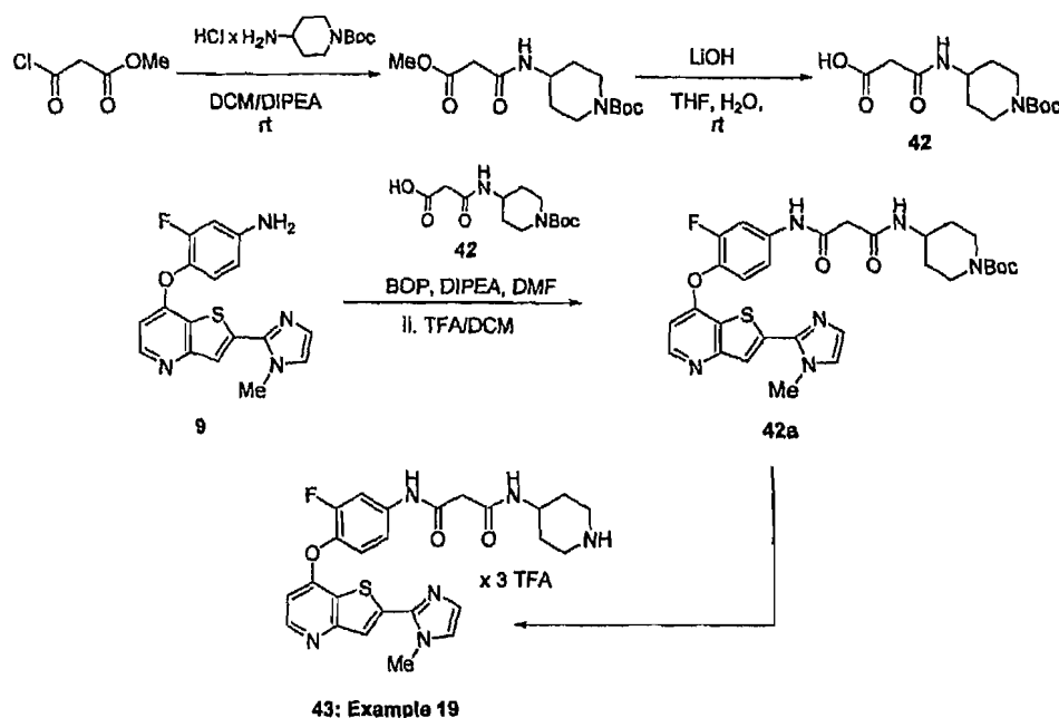
Scheme 15
