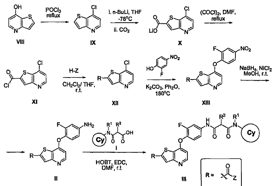
Scheme C
