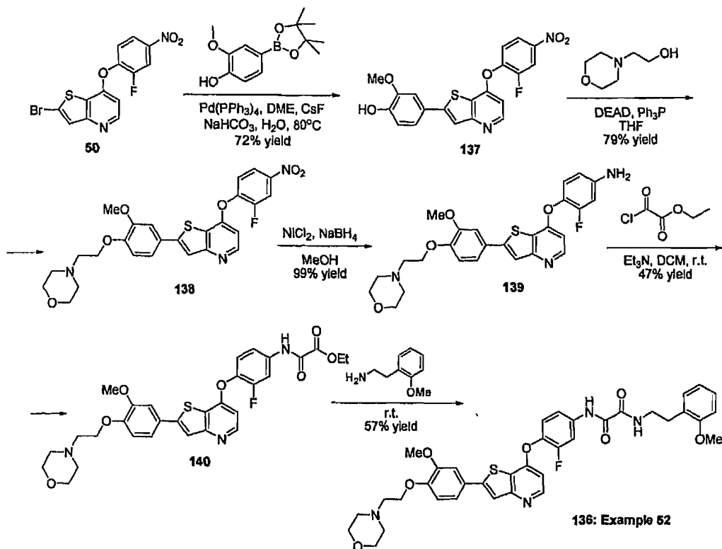
Scheme 40
