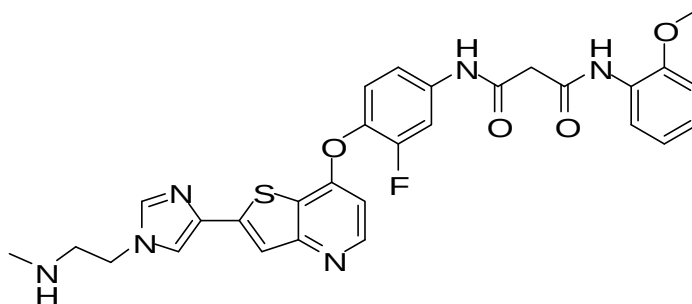
N 1 -(4-(2-(1 H -imidazol-4-yl)thieno[3,2- b ]pyridin-7-yloxy)-3-fluorophenyl)- N 3 -(2-methoxyphenyl)malonamide,
