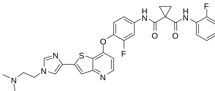
N -(3-fluoro-4-(2-(1-(3-(pyrrolidin-1-yl)propyl)-1 H -imidazol-4-yl)thieno[3,2- b ]pyridin-7-yloxy)phenyl)- N -(2-fluorophenyl)cyclopropane-1,1-dicarboxamide,
