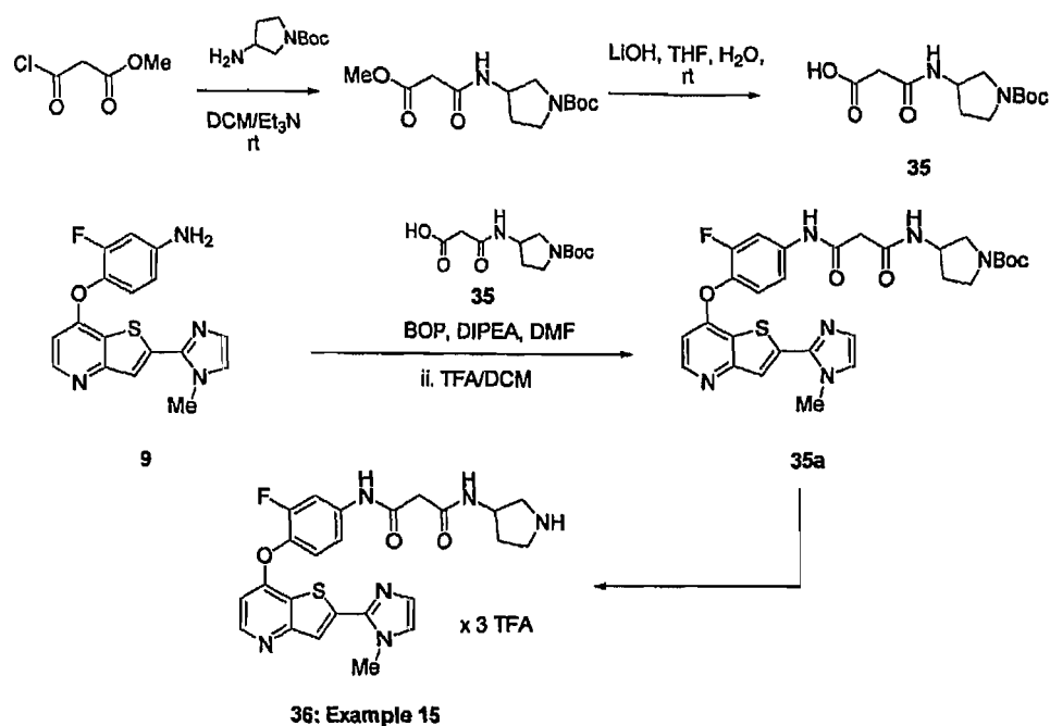
Scheme 12
