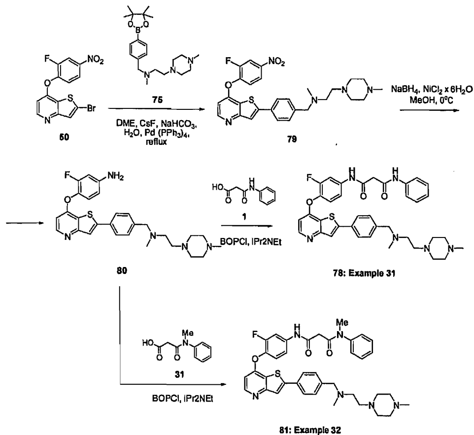
Scheme 26
