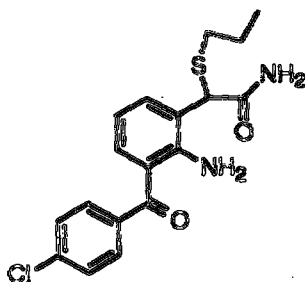
Compound 3 2-Amino-3-(4-chlorobenzoyl)- \alpha -(n-propylthio)-phenylacetamide
