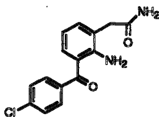
Compound 9 2-Amino-3-(4-chlorobenzoyl)-phenylacetamide
