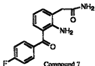
Compound 7 2-Amino-3-(4-fluorobenzoyl)-phenylacetamide
