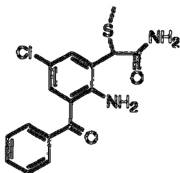
Compound 4 2-Amino-3-benzoyl-5-chloro- \alpha -(methylthio)-phenylacetamide
