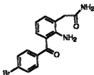
Compound 15 2-Amino-3-(4-bromobenzoyl)-phenylacetamide
