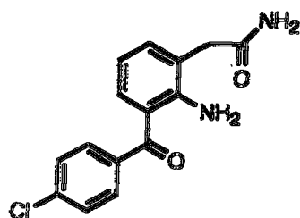
Compound 9 2-Amino-3-(4-chlorobenzoyl)-phenylacetamide
