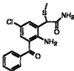
Compound 4
