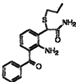
Compound 2 2-Amino-3-benzoyl- \alpha -(n-propylthio)-phenylacetamide
