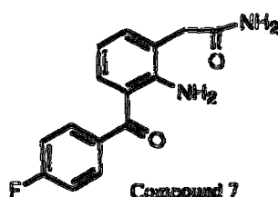
Compound 7
