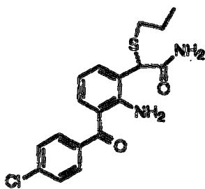
Compound 3 2-Amino-3-(4-chlorobenzoyl)- \alpha -(n-propylthio)-phenylacetamide
