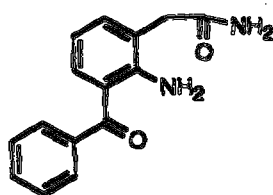
Compound 8
