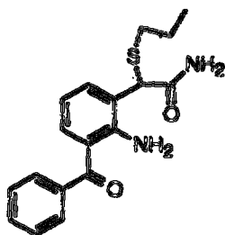
Compound 2 2-Amino-3-benzoyl- \alpha -(n-propylthio)-phenylacetamide
