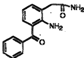
Compound 8 2-Amino-3-benzoyl-phenylacetamide
