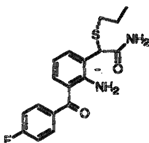
Compound 1 2-Amino-3-(4-fluorobenzoyl)- \alpha -(n-propylthio)-phenylacetamide
