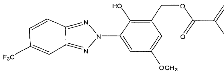
Compound WL-1
