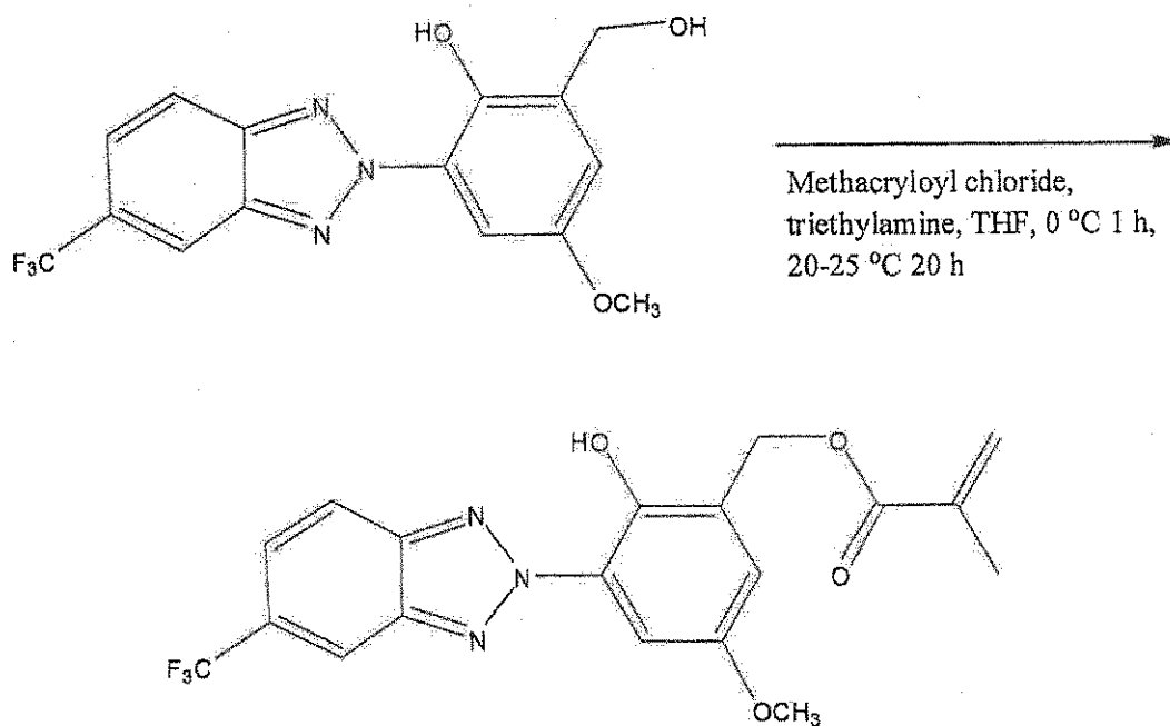
Compound WL-1
