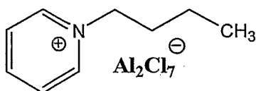
1-Butyl-pyridinium heptachloroaluminate
