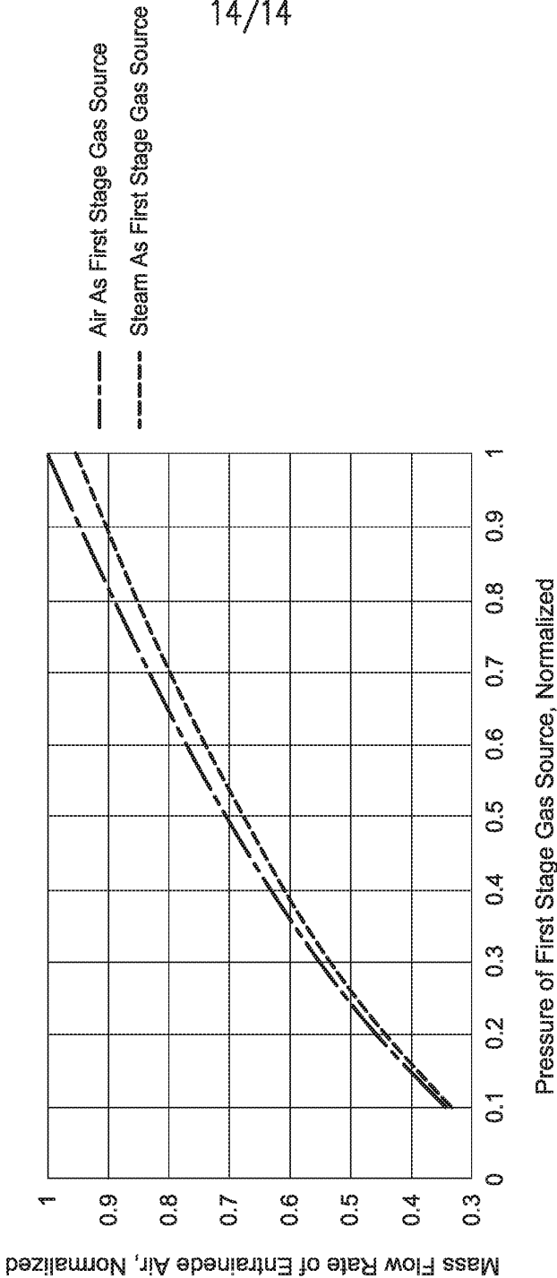
Computer Model Simulation of Air Entrainment Performance Using Steam And Air as the First Stage Gas Source
