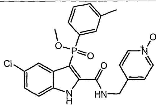
Compound J
