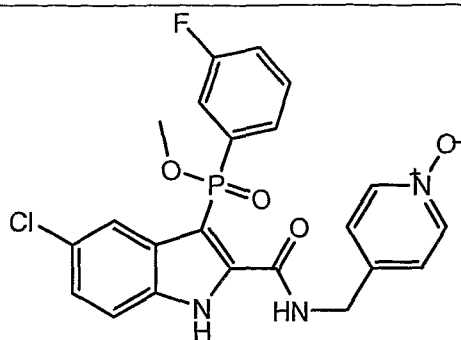
Compound I
