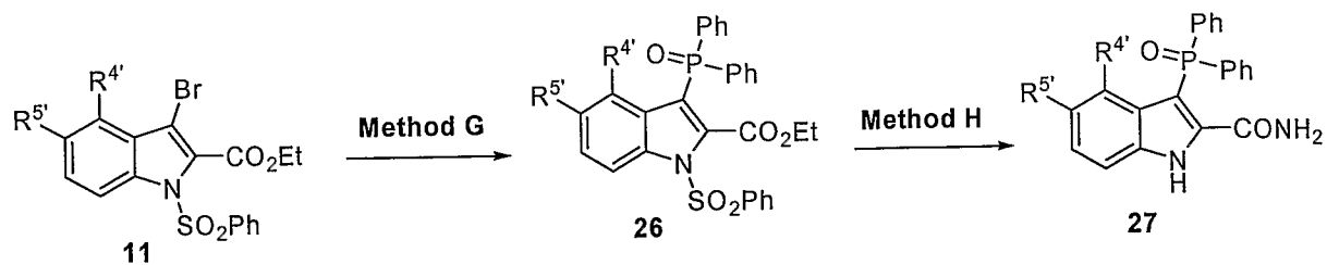
Scheme 7:
