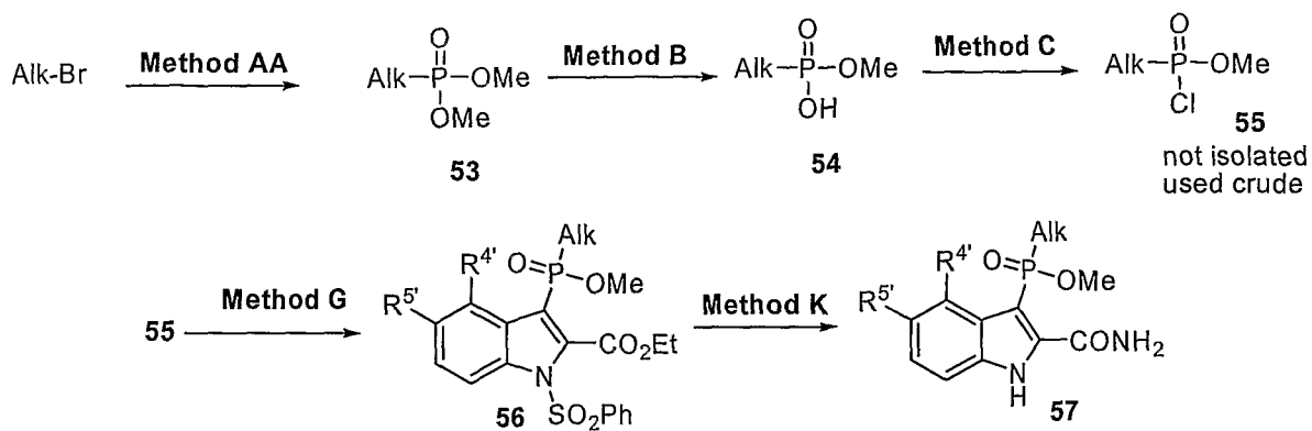
Scheme 14: Alkyl Phosphinates
