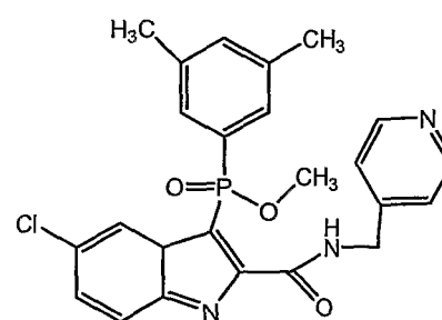
Compound N
