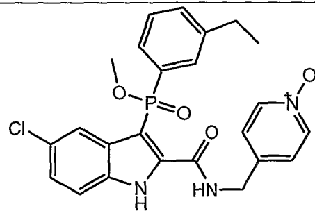
Compound L
