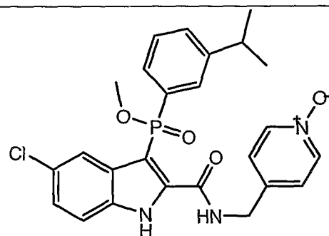
Compound M
