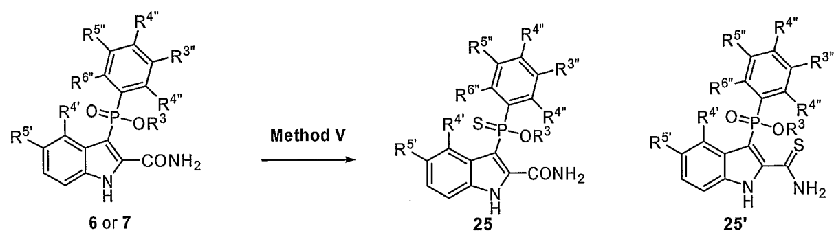
Scheme 5:
