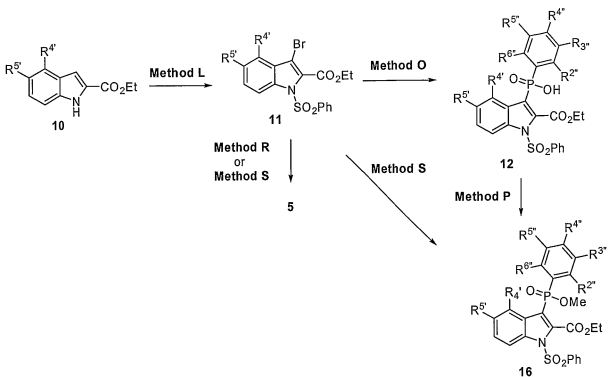
Scheme 4:
