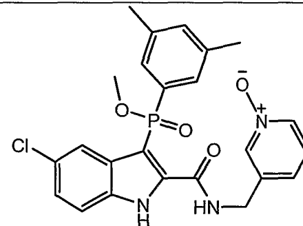
Compound F
