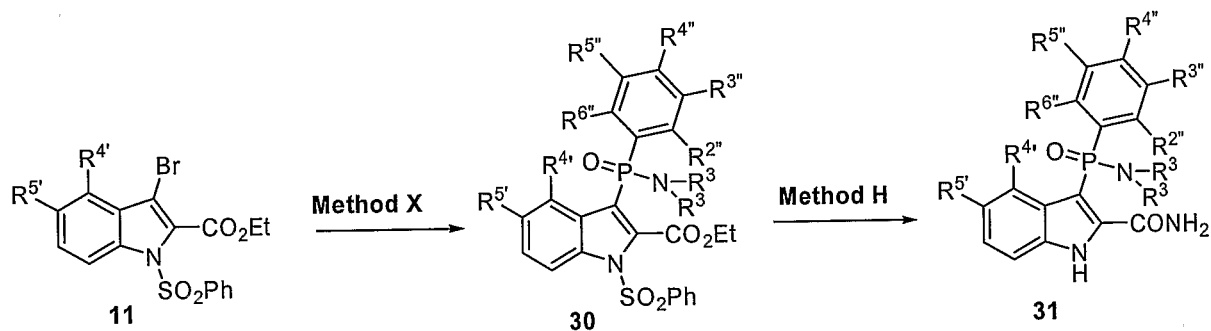
Scheme 8:
