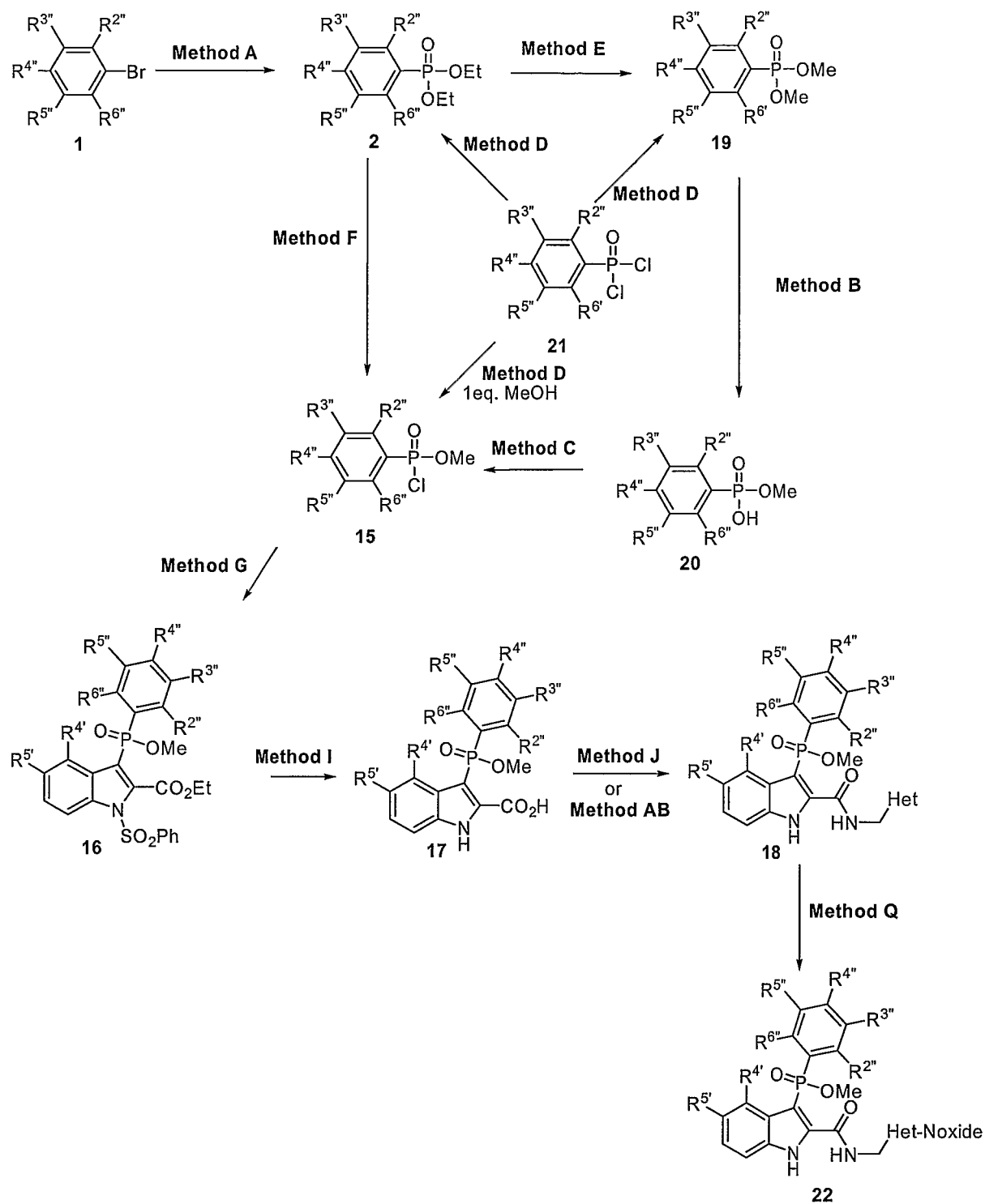
Scheme 2:
