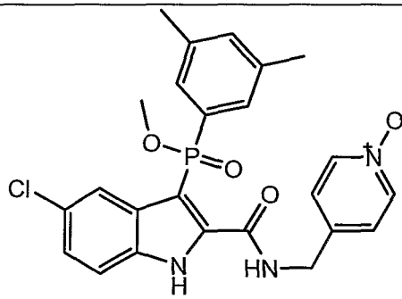
Compound D
