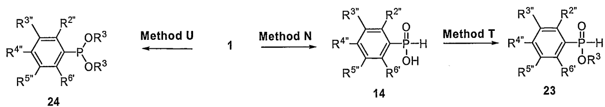
Scheme 4:
