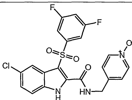
Compound H
