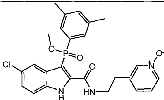
Compound E
