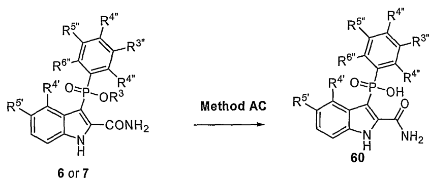
Scheme 16: Phosphinic Acids
