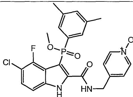
Compound B
