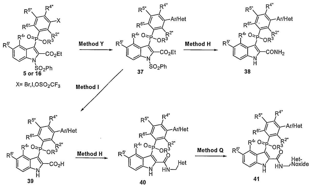
Scheme 10:
