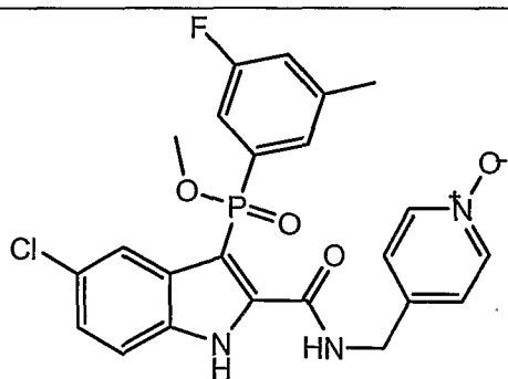
Compound G
