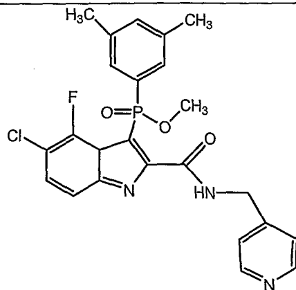
Compound M
