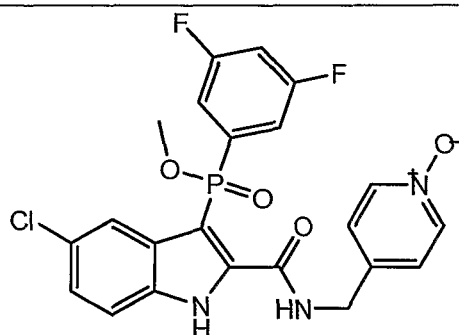
Compound C
