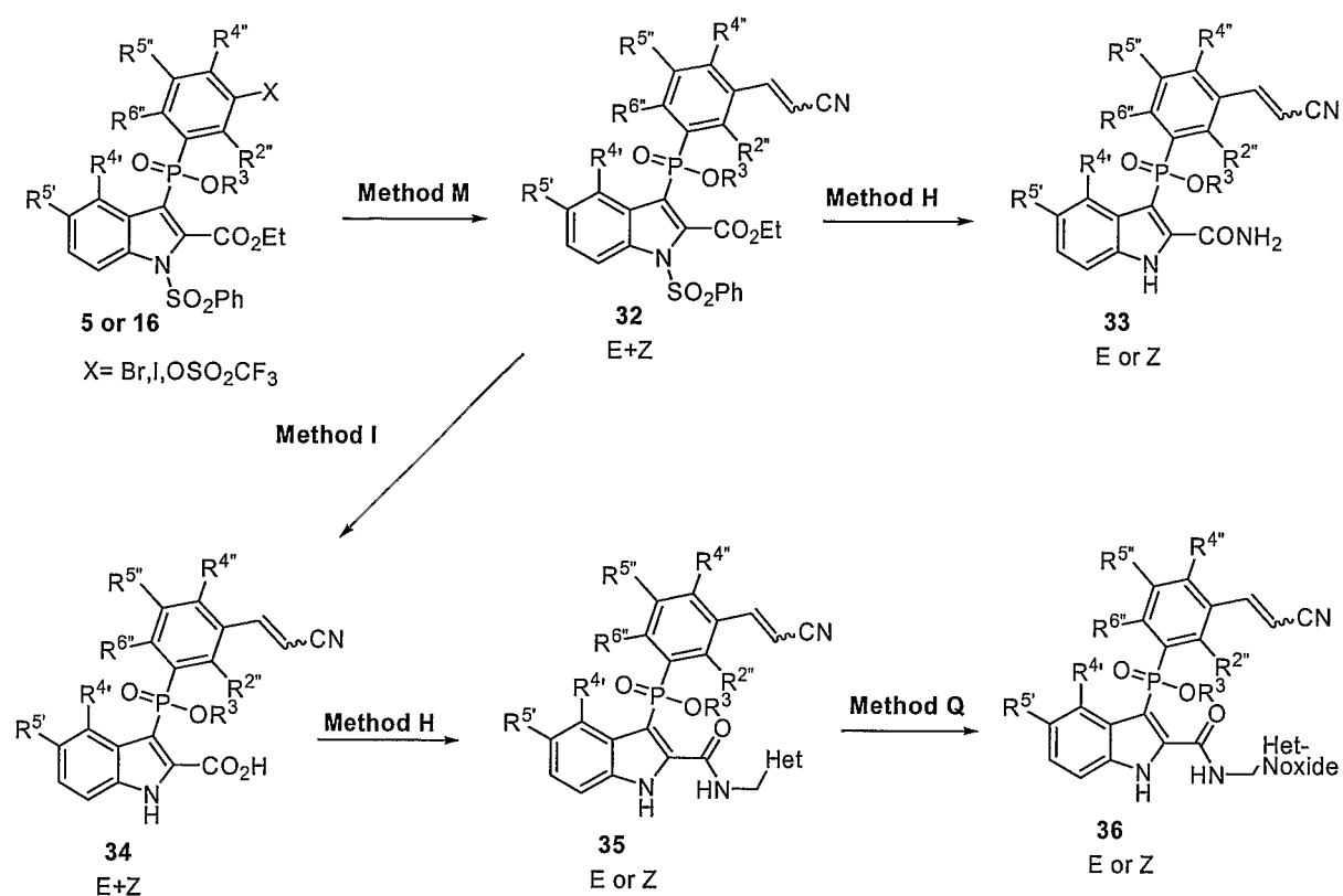
Scheme 10:
