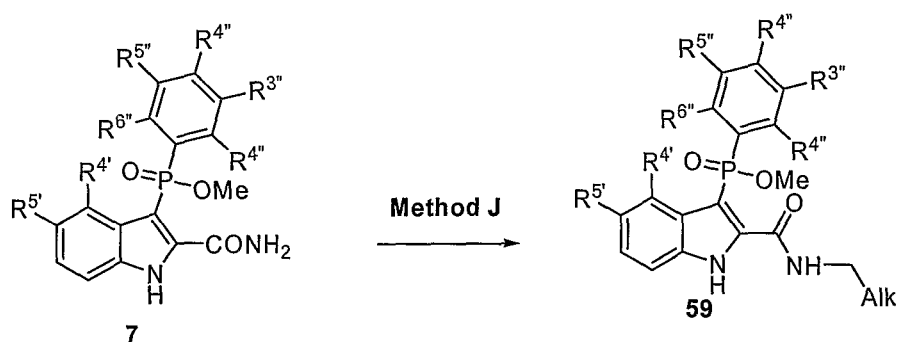
Scheme 16: Phosphinic Acids
