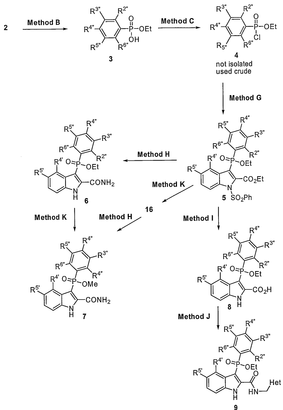
Scheme 3:
