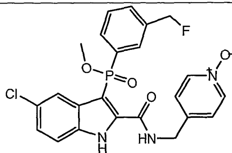
Compound K
