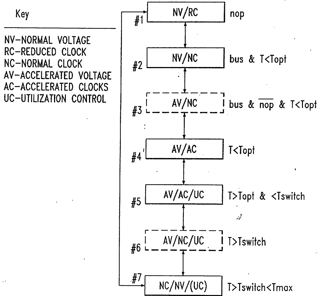
Switching control flow diagram
