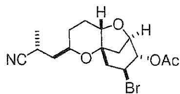
Compound AK
