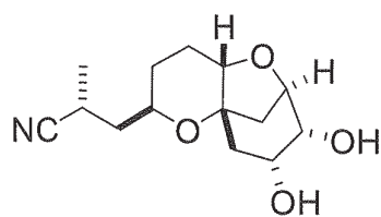
Compound AJ
