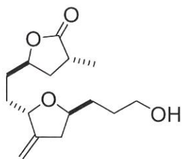
Compound AR.
