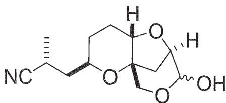
Compound AM.
