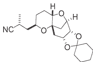
Compound AD
