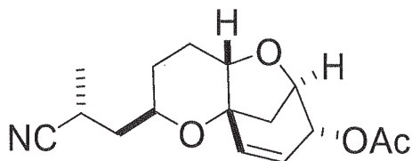
Compound AL.
