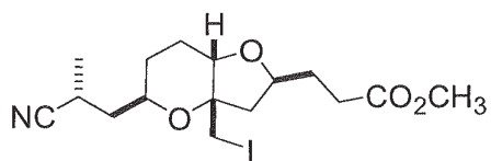
Compound AF.
