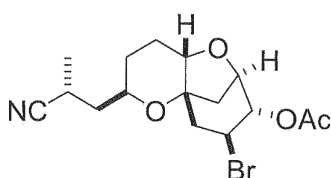
Compound AK
