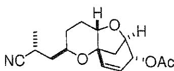
Compound AL
