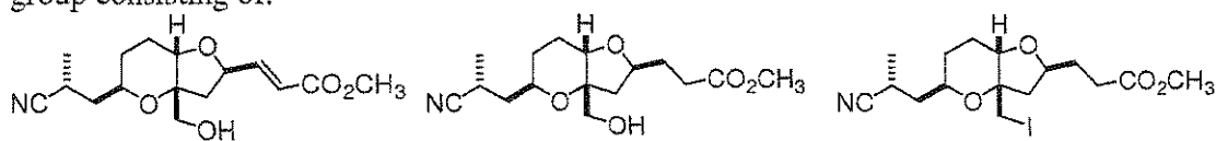
Compound AO
