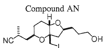
Compound AN
