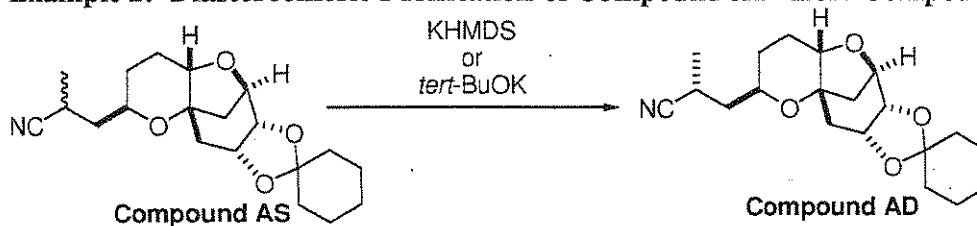
Scheme 12
