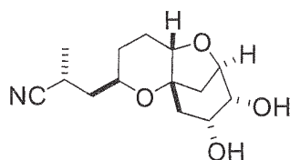
Compound AJ
