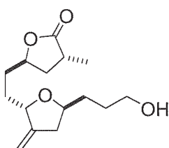
Compound AR.
