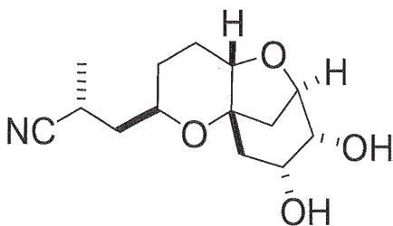
Compound AJ
