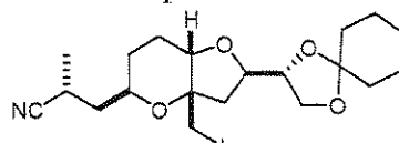
Compound AO
