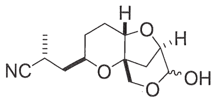
Compound AM.
