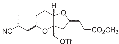
Compound AT
