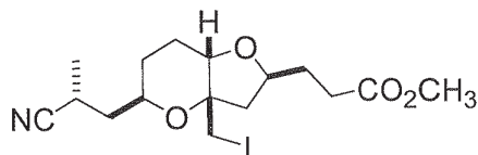
Compound AF.
