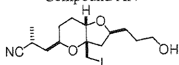
Compound AN
