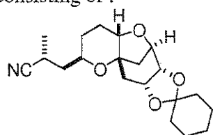
Compound AD
