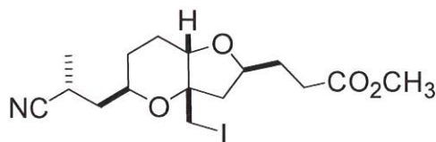
Compound AF.
