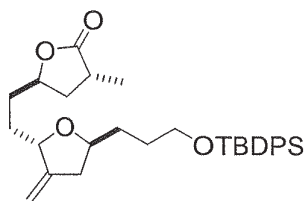
Compound AH.
