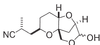
Compound AM.
