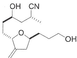
Compound AU.
