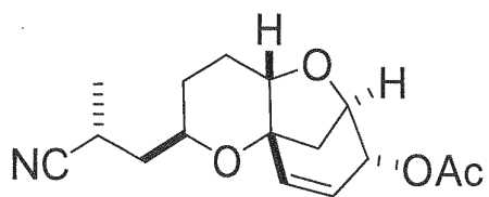
Compound AL
