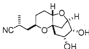
Compound AJ
