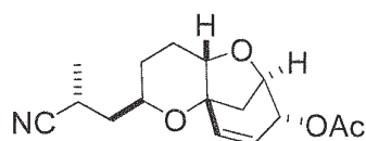
Compound AL
