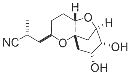
Compound AJ
