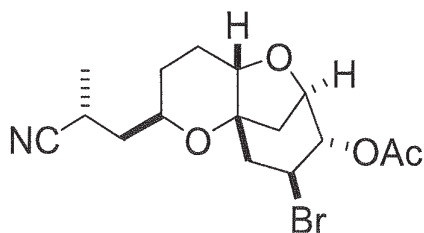
Compound AK
