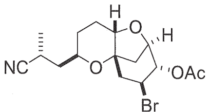
Compound AK.
