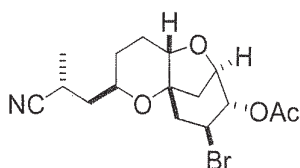
Compound AK.
