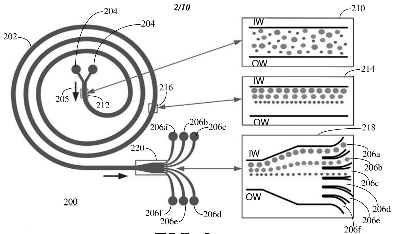
FIG. 2 PRIOR ART
