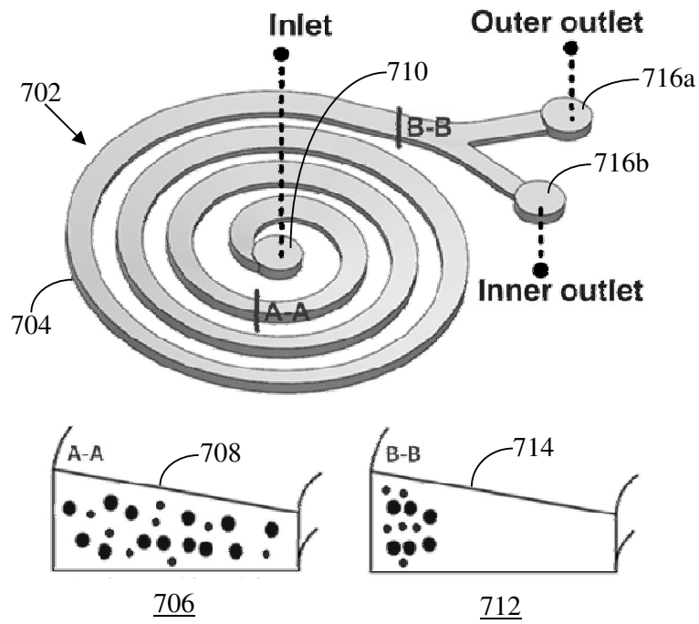
FIG. 7 PRIOR ART
