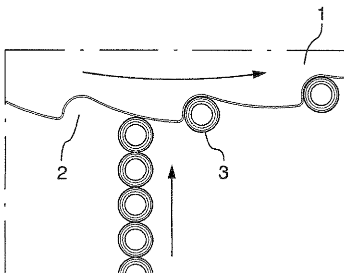
FIG. 18 (Prior Art)
