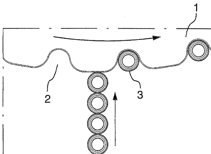
FIG. 17 (Prior Art)
