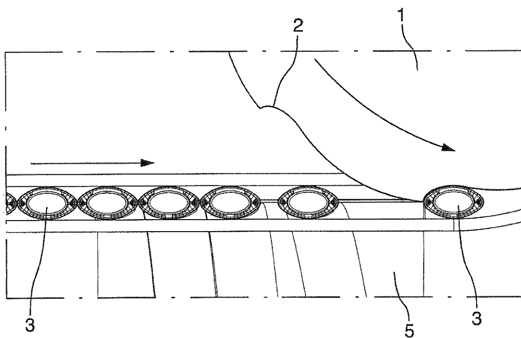
FIG.19 (Prior Art)
