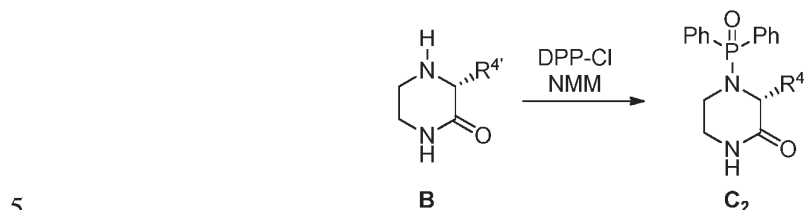
Scheme 9 : DPP protection of B .
