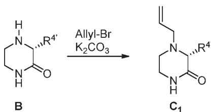
Scheme 8: Allyl protection of B.
