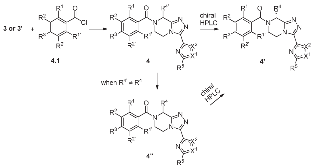
Scheme 6: Acylation and chiral HPLC purification.
