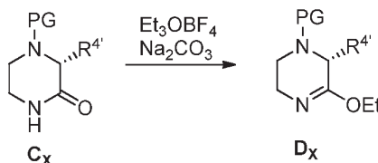
Scheme 12: Conversion to iminoether D .
