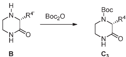
Scheme 10 : Boc protection of B .
