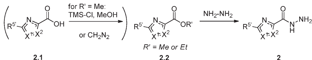
Scheme 4: Formation of acylhydrazide 2.
