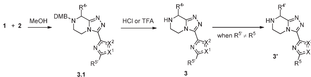
Scheme 5: Cyclodehydration leading to triazolopiperazine 3.
