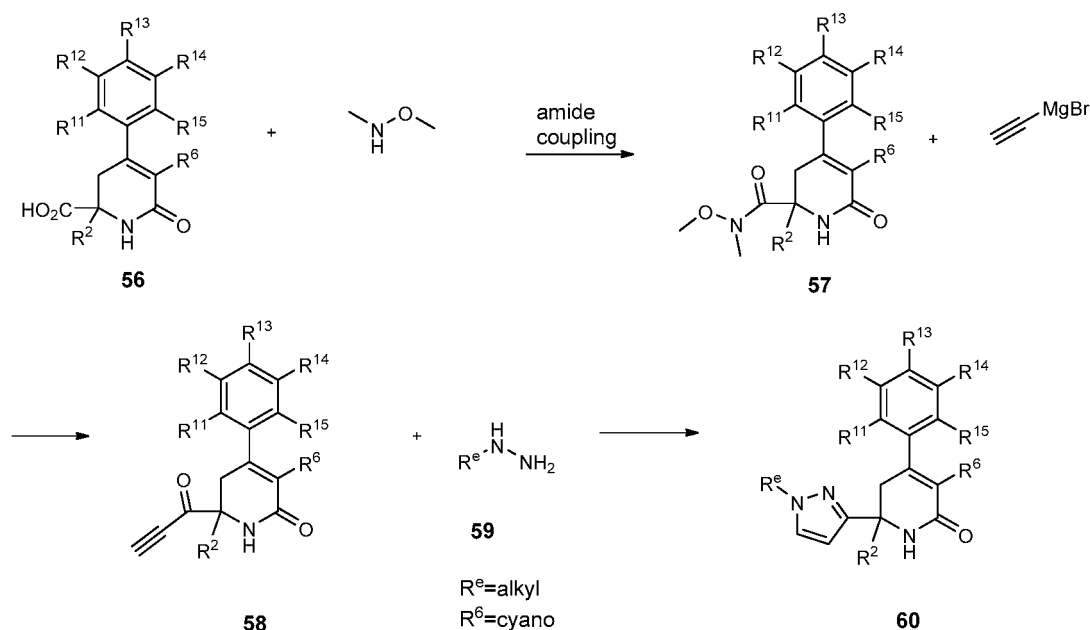
Scheme 15
