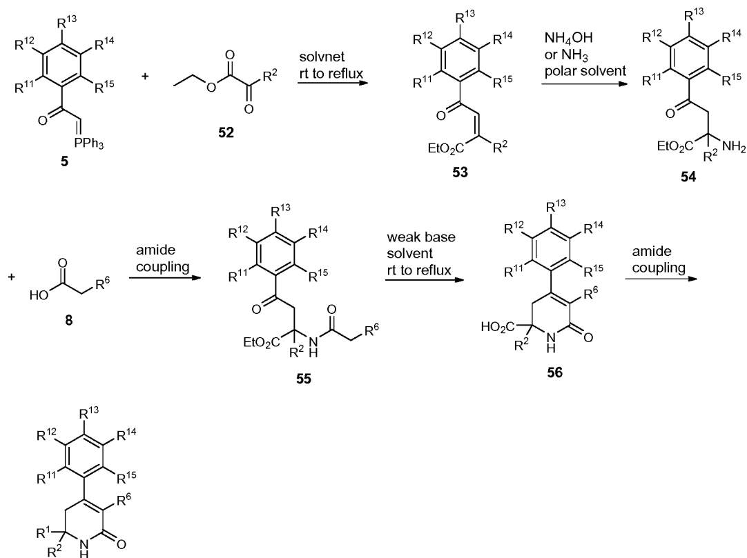
Scheme 14
