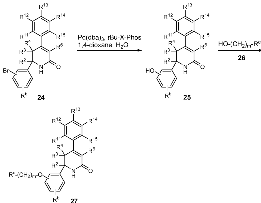
Scheme 7
