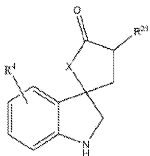
Formula (XXVIIIf);
