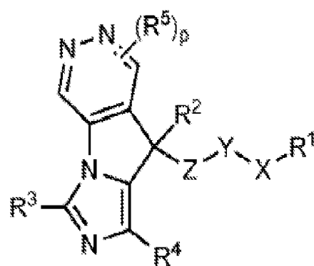
Formula (XLIXh);
