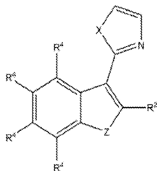
Formula (XXVa);
