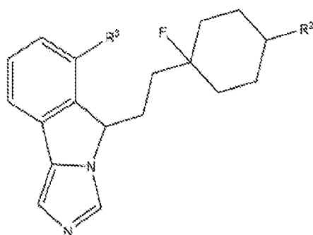
Formula (XXXab).
