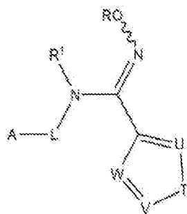
Formula (XIII).
