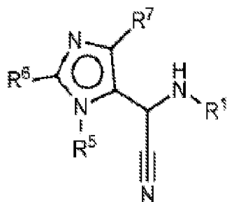
Formula (XLVm);
