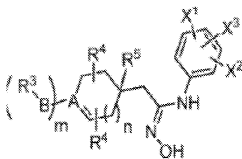
Formula (LVb);
