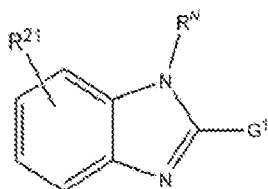
Formula (XXVIIIf);
