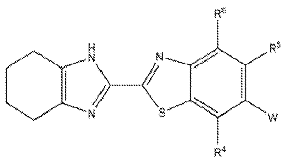
Formula (XIXn);
