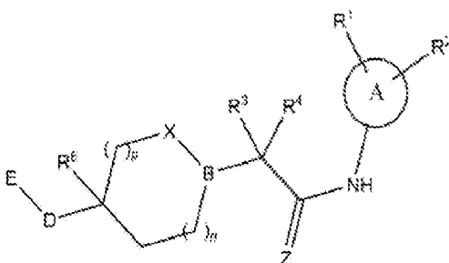
Formula (XLIIIb);
