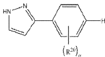
Formula (IXs);
