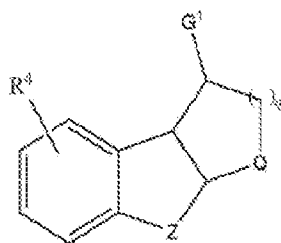
Formula (XXVIf);
