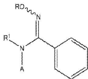
Formula (XVIIb);
