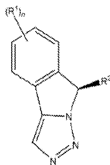
Formula (XXIXg);
