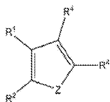
Formula (XXVIIIp);
