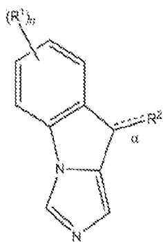
Formula (XXIXa);
