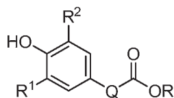
(Formula II),
