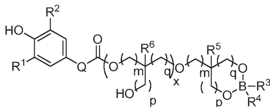
Formula (IV)
