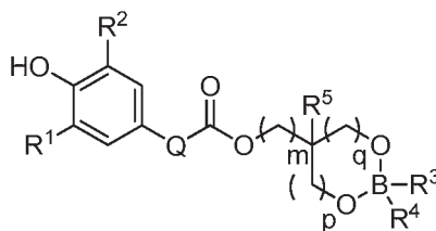
Formula (VI)
