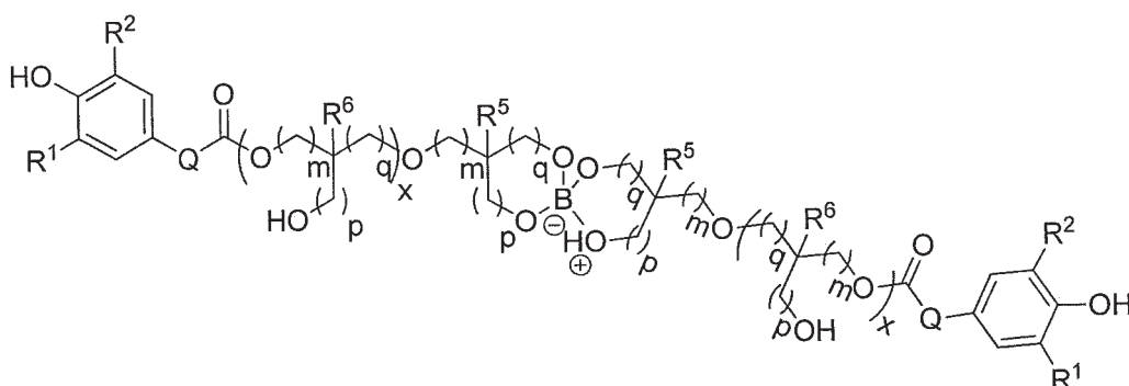
Formula (V)
