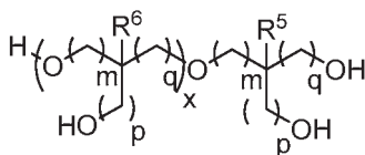
(Formula III),
