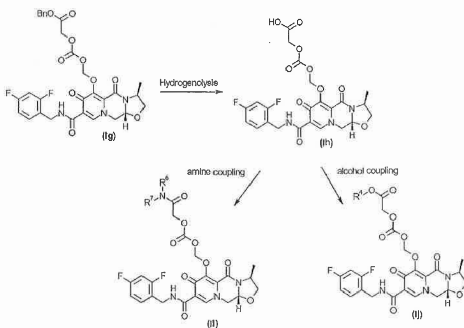
Scheme 5
