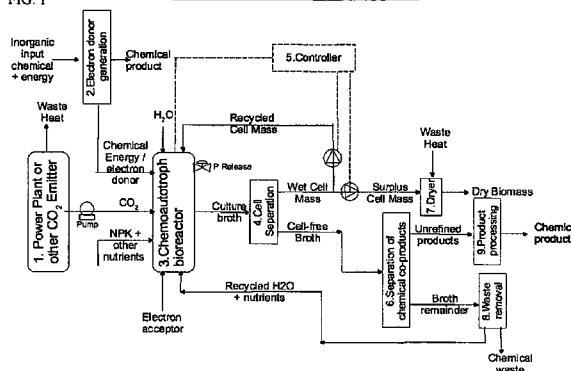
General Process Flow Diagram
