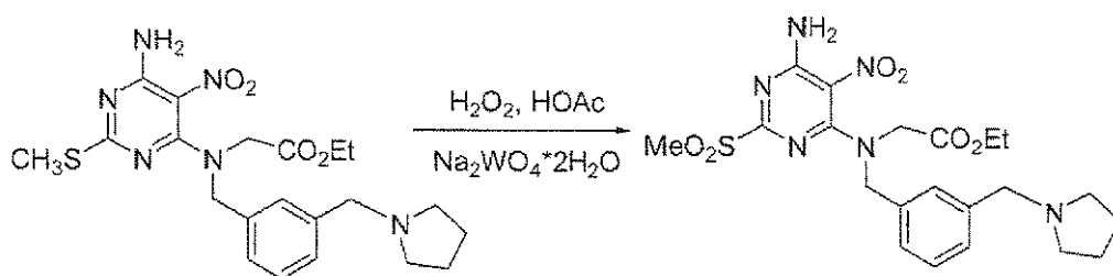
Scheme 11
