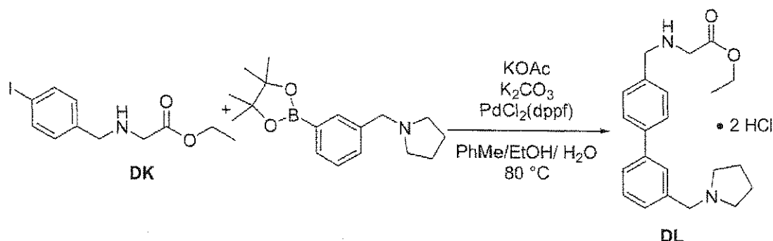
Scheme 78
