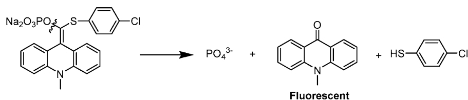
Scheme 1. CPA
