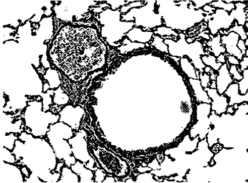
Viable LGG
