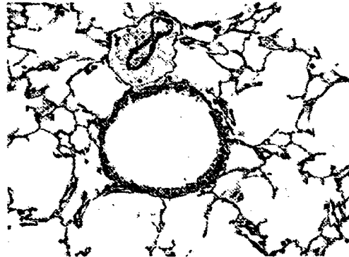
LGG Supernatant
