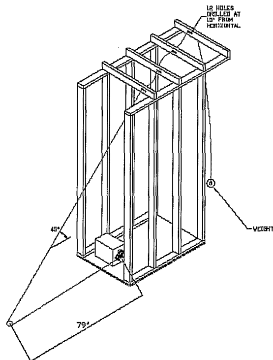
Modified Joist-Pull Test
