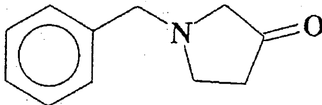
N-Benzyl-3-pyrrolidinone
