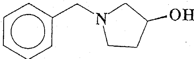
(S)-N-Benzyl-3-pyrrolidinol
