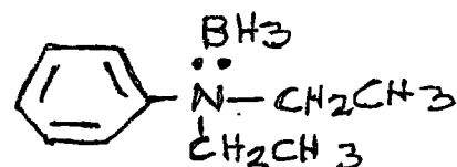
N,N-diethylaniline borane
