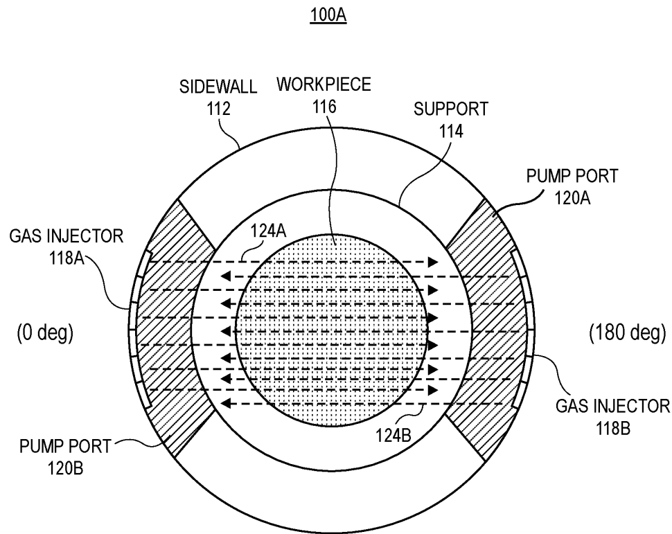
2-Phase Cross-flow Operation
